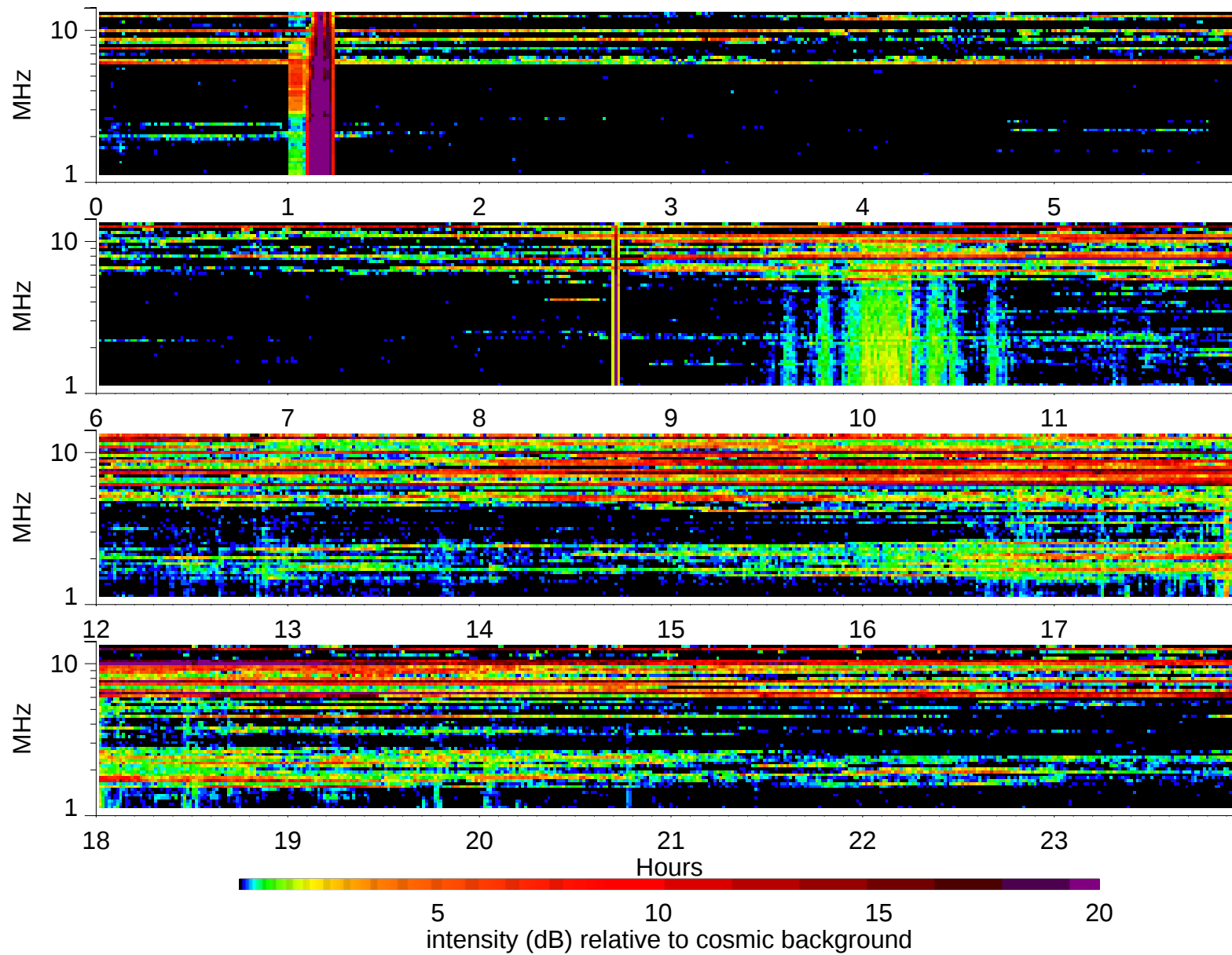
Wind Waves RAD2 receiver: 1995/12/20
