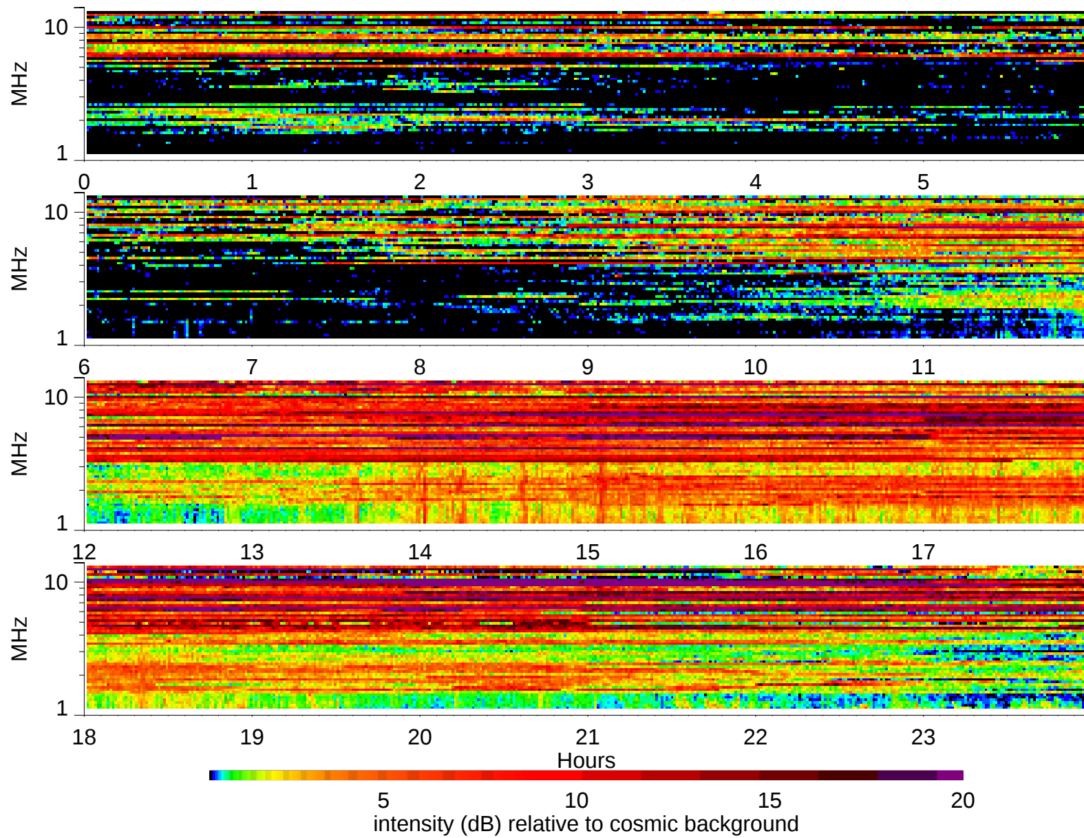
Wind Waves RAD2 receiver: 1995/12/21
