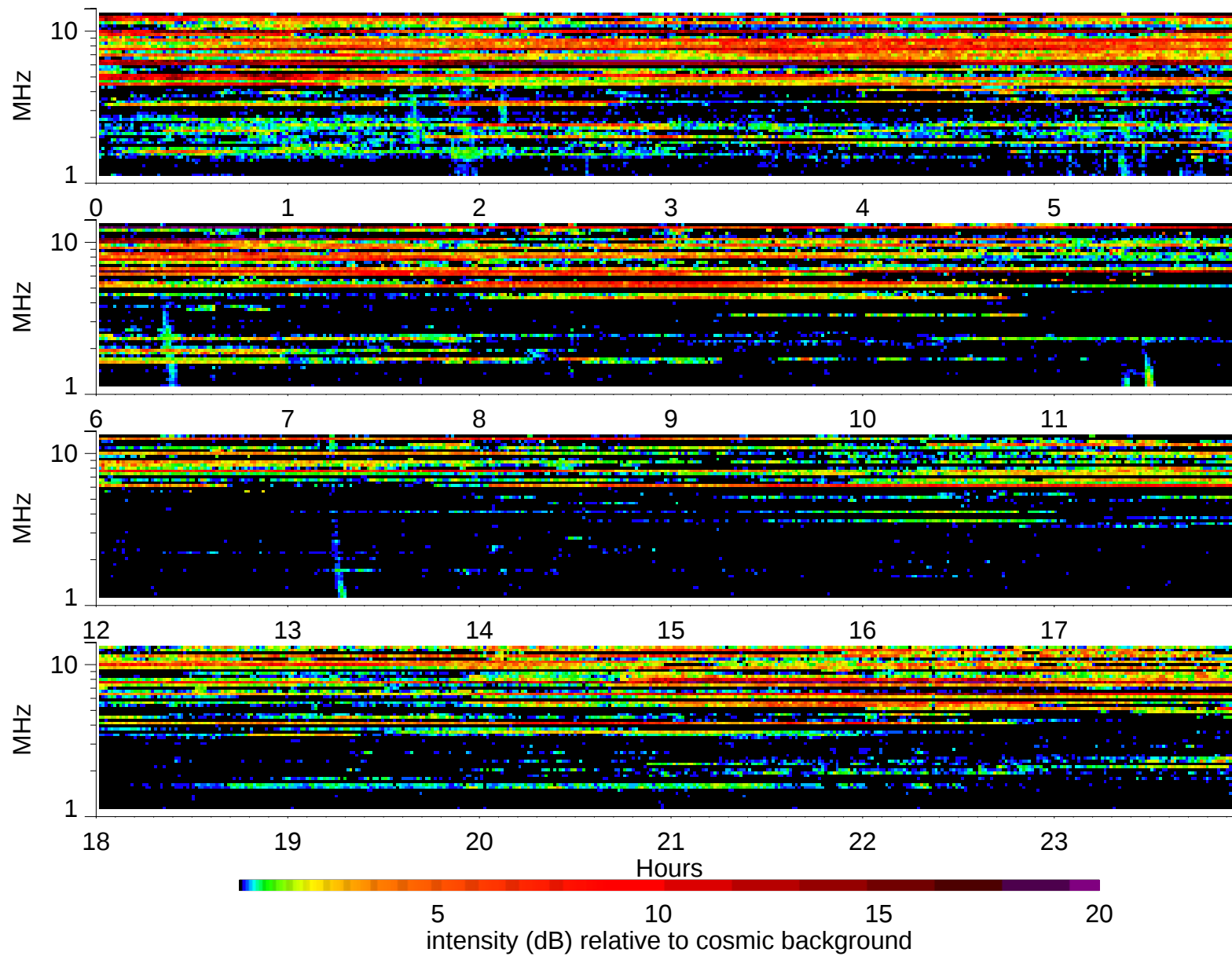
Wind Waves RAD2 receiver: 1995/12/23
