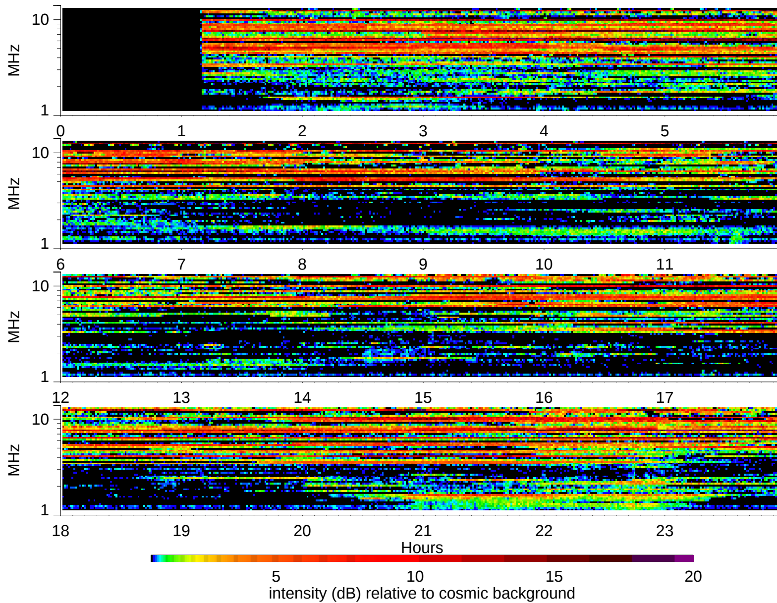
Wind Waves RAD2 receiver: 1997/1/1
