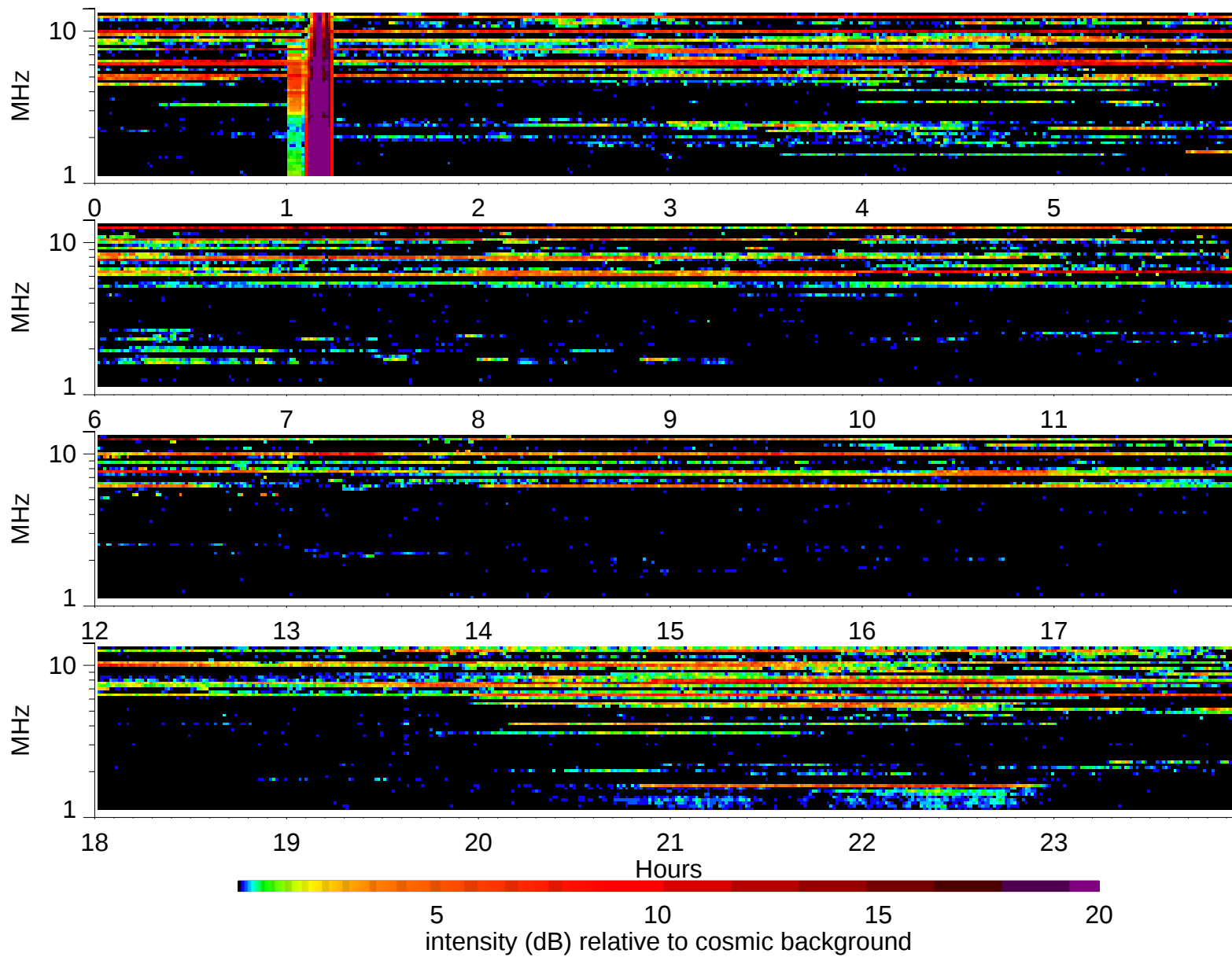
Wind Waves RAD2 receiver: 1997/1/6
