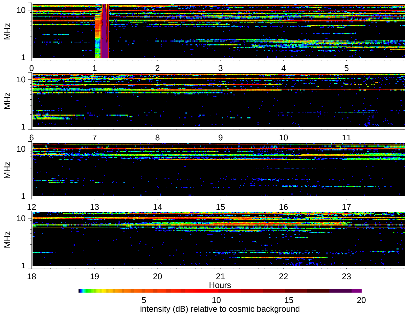
Wind Waves RAD2 receiver: 1997/1/8
