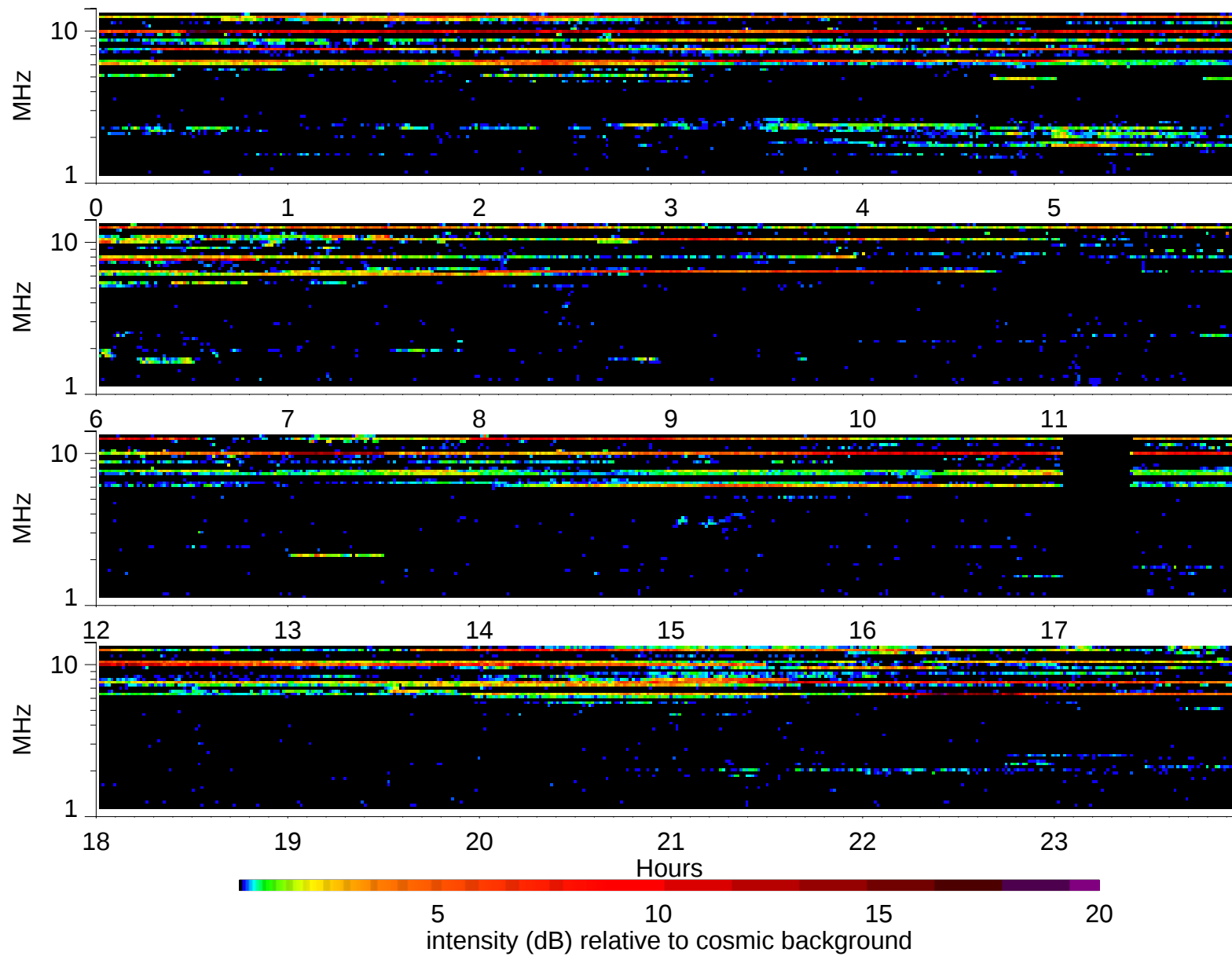
Wind Waves RAD2 receiver: 1997/1/9
