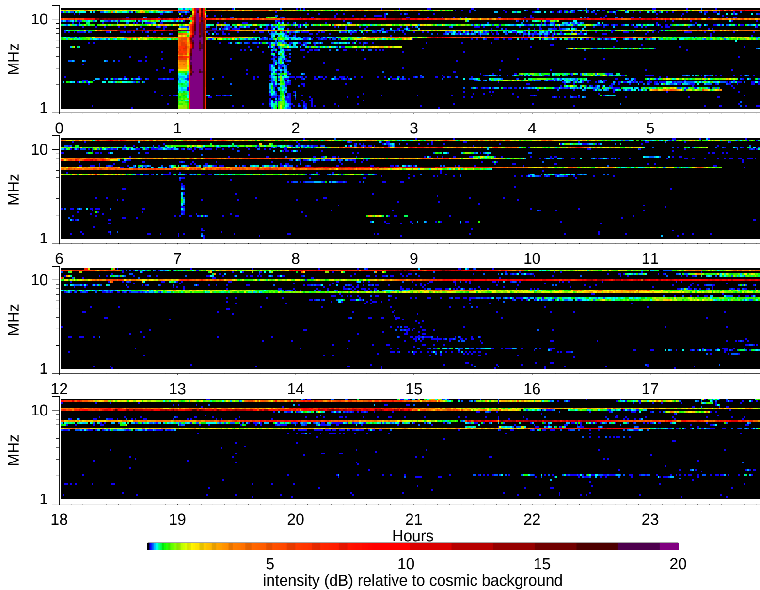
Wind Waves RAD2 receiver: 1997/1/10
