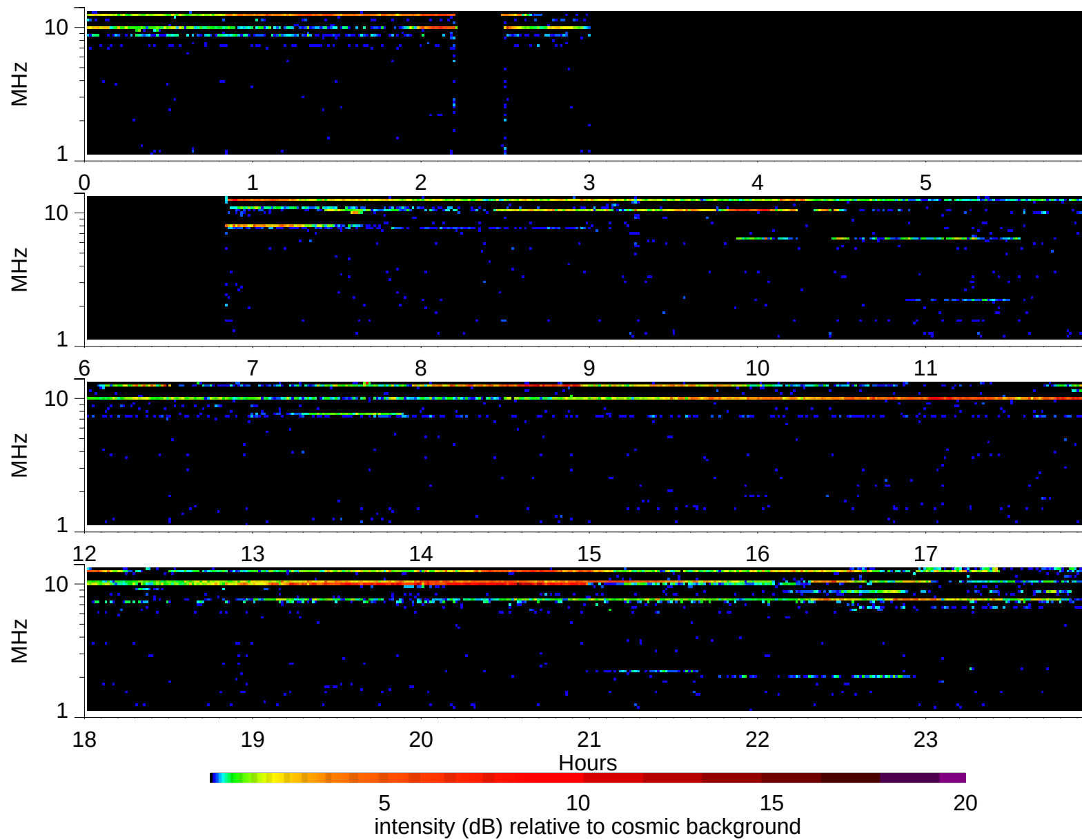
Wind Waves RAD2 receiver: 1997/1/13
