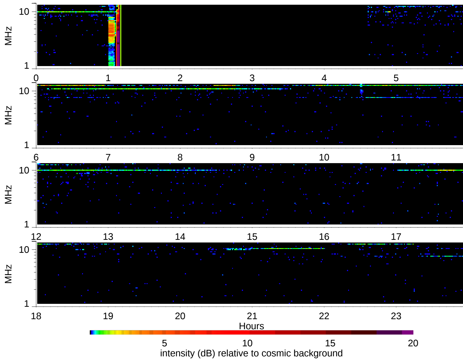
Wind Waves RAD2 receiver: 1997/1/24
