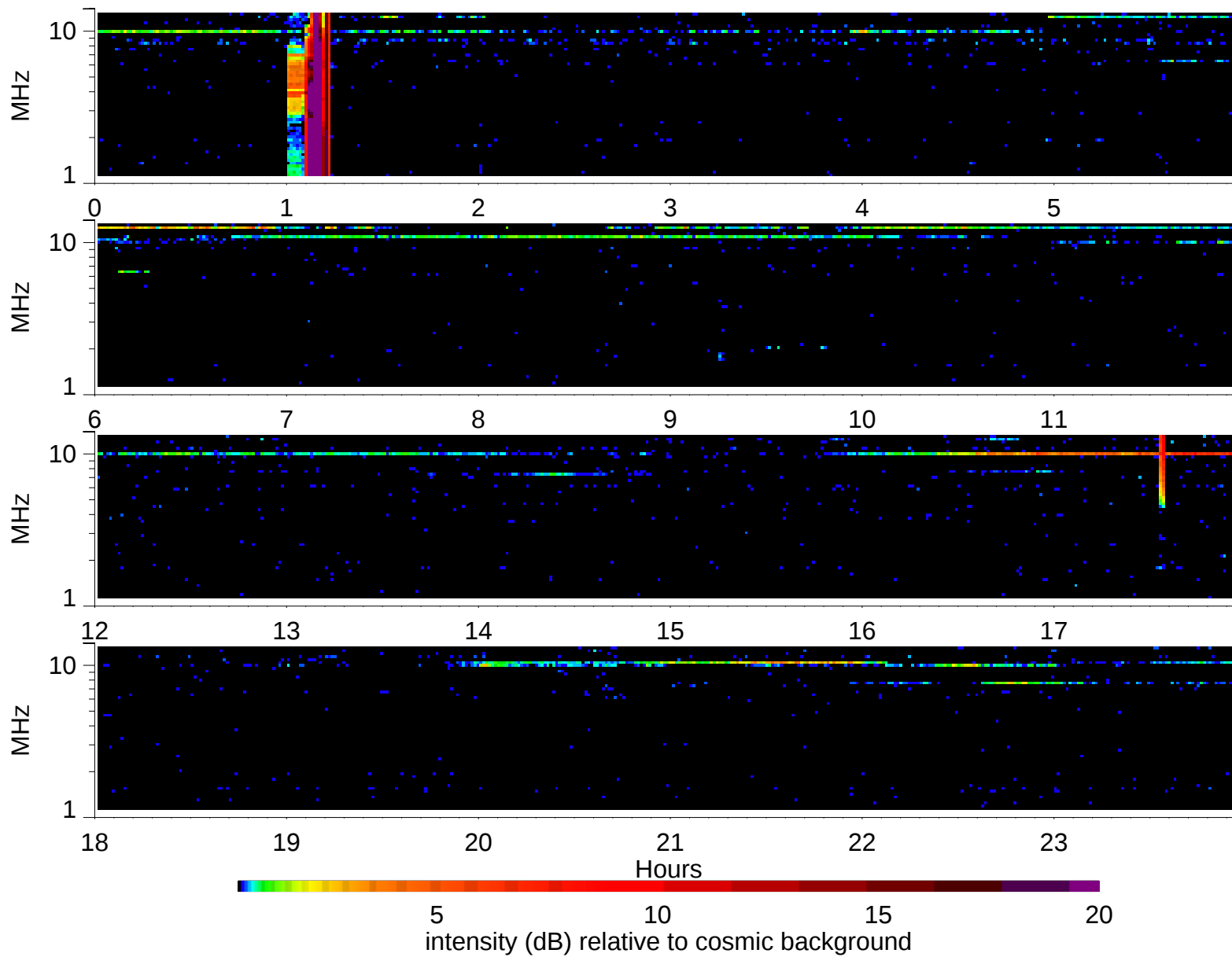
Wind Waves RAD2 receiver: 1997/1/28
