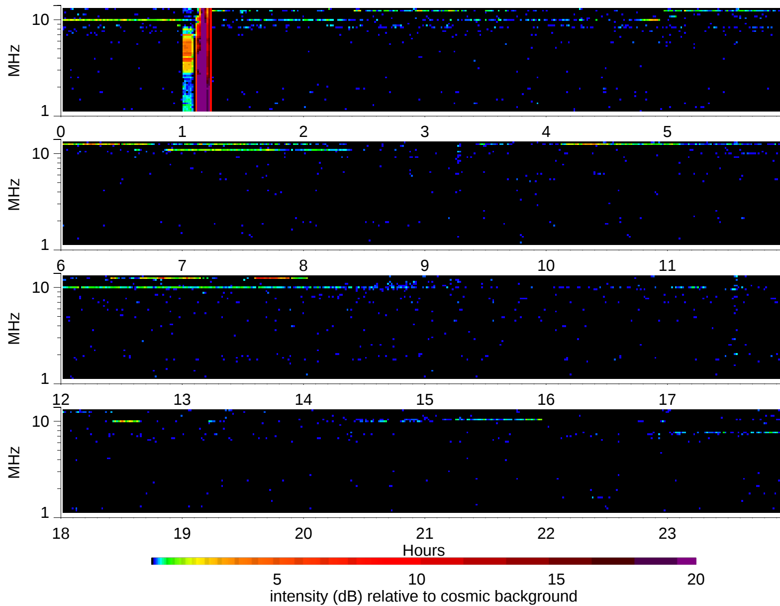
Wind Waves RAD2 receiver: 1997/1/30
