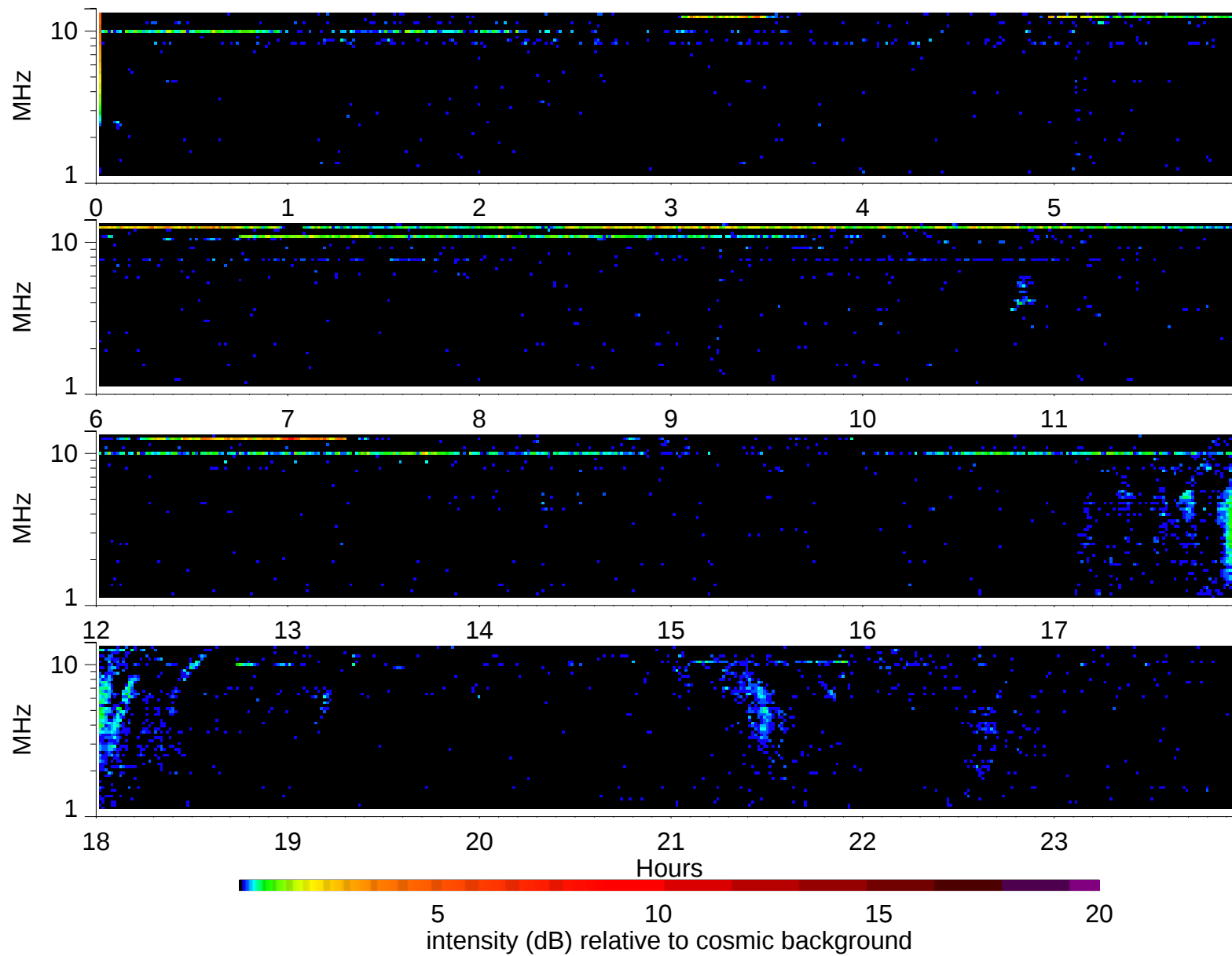
Wind Waves RAD2 receiver: 1997/1/31
