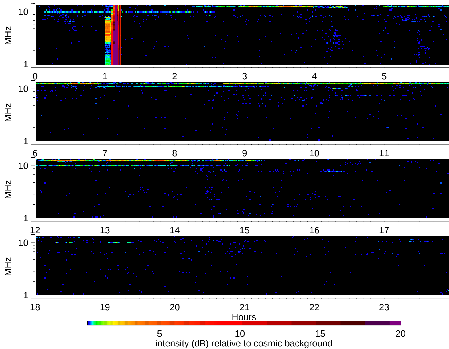
Wind Waves RAD2 receiver: 1997/2/5
