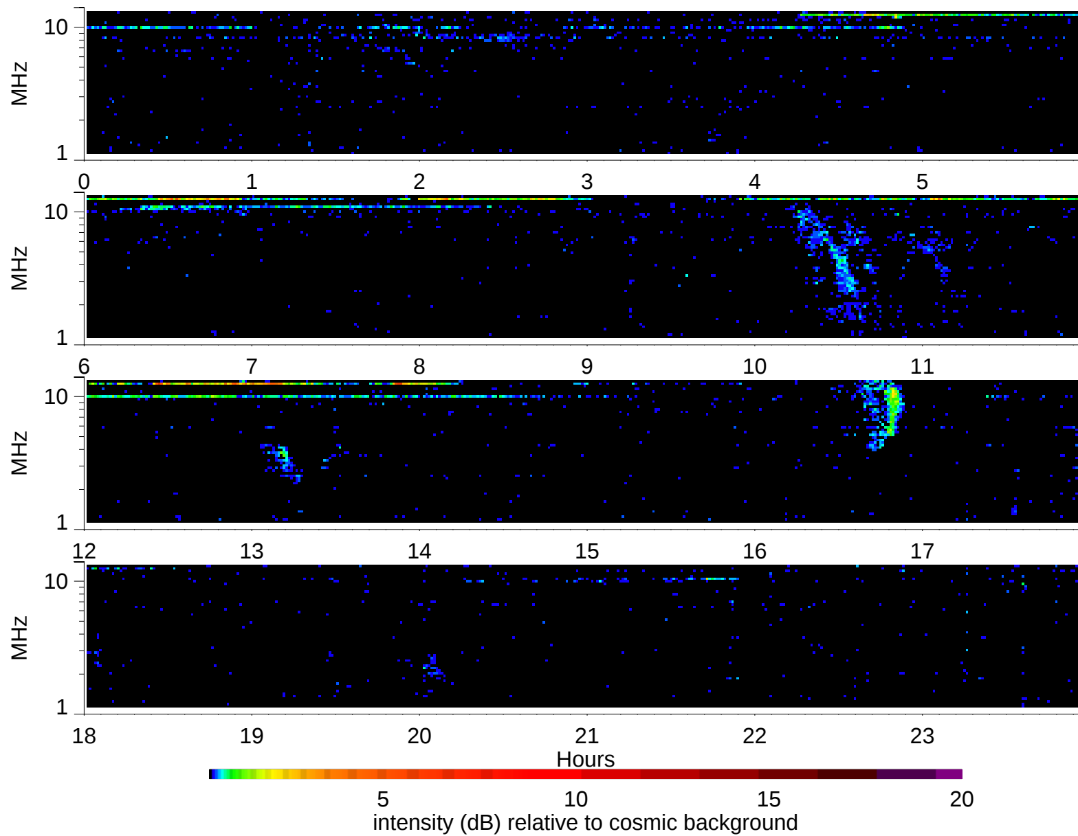
Wind Waves RAD2 receiver: 1997/2/6
