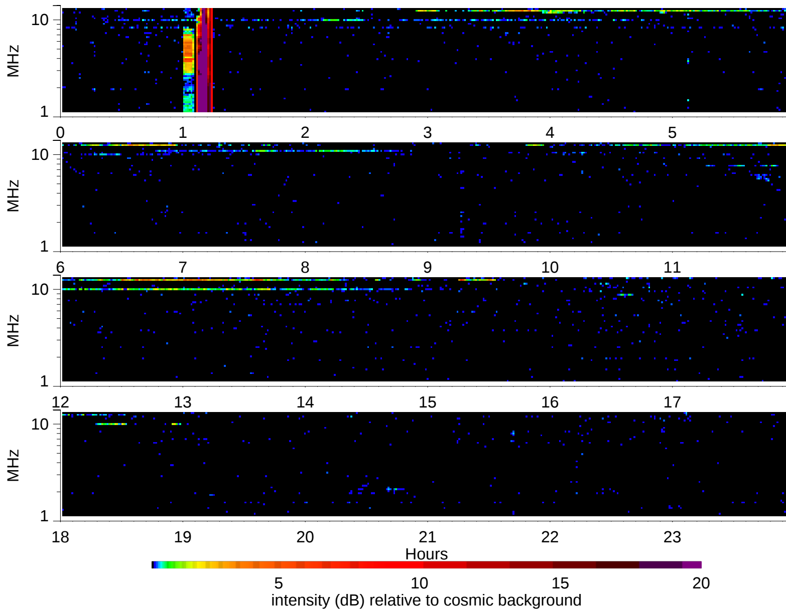
Wind Waves RAD2 receiver: 1997/2/7
