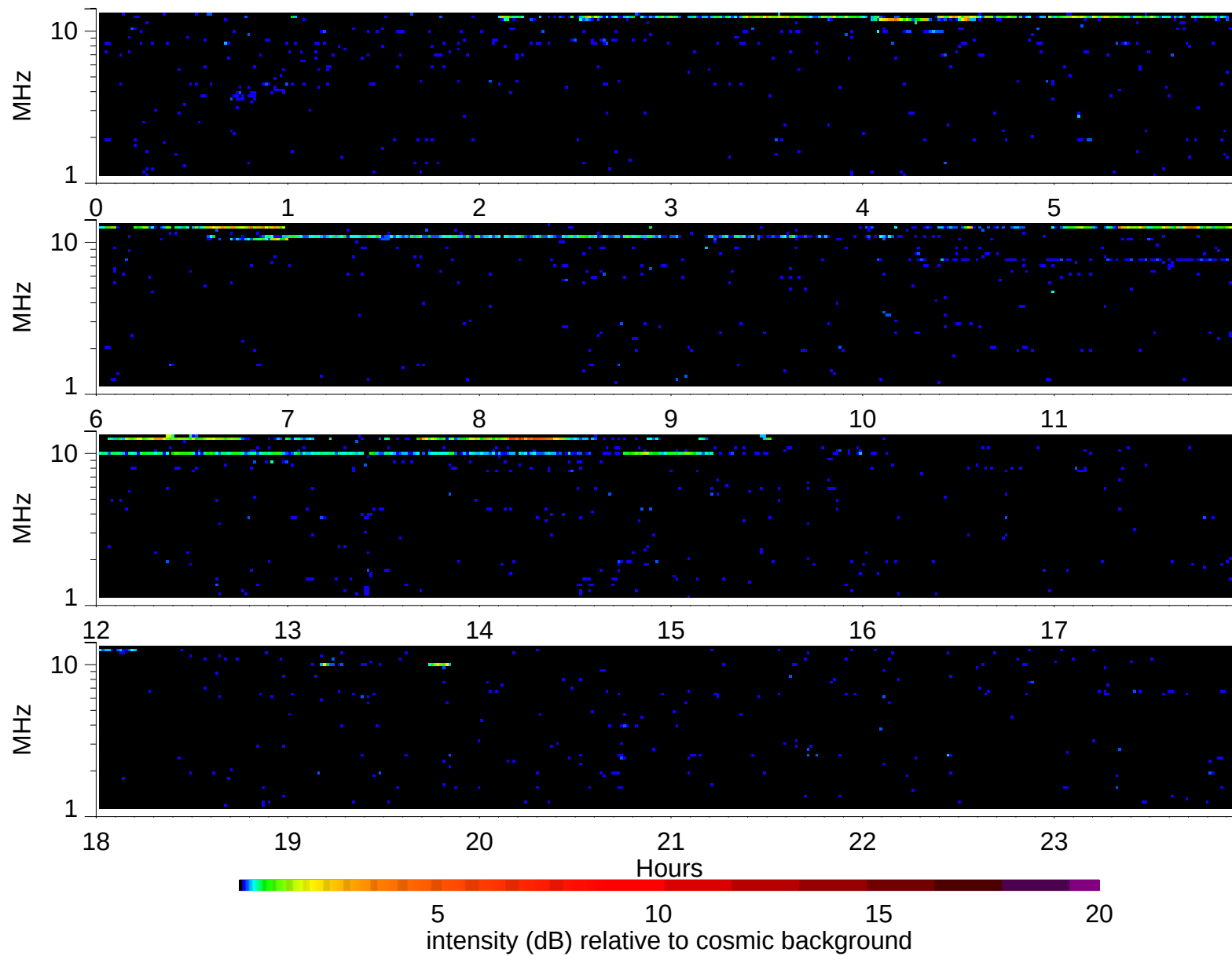
Wind Waves RAD2 receiver: 1997/2/12
