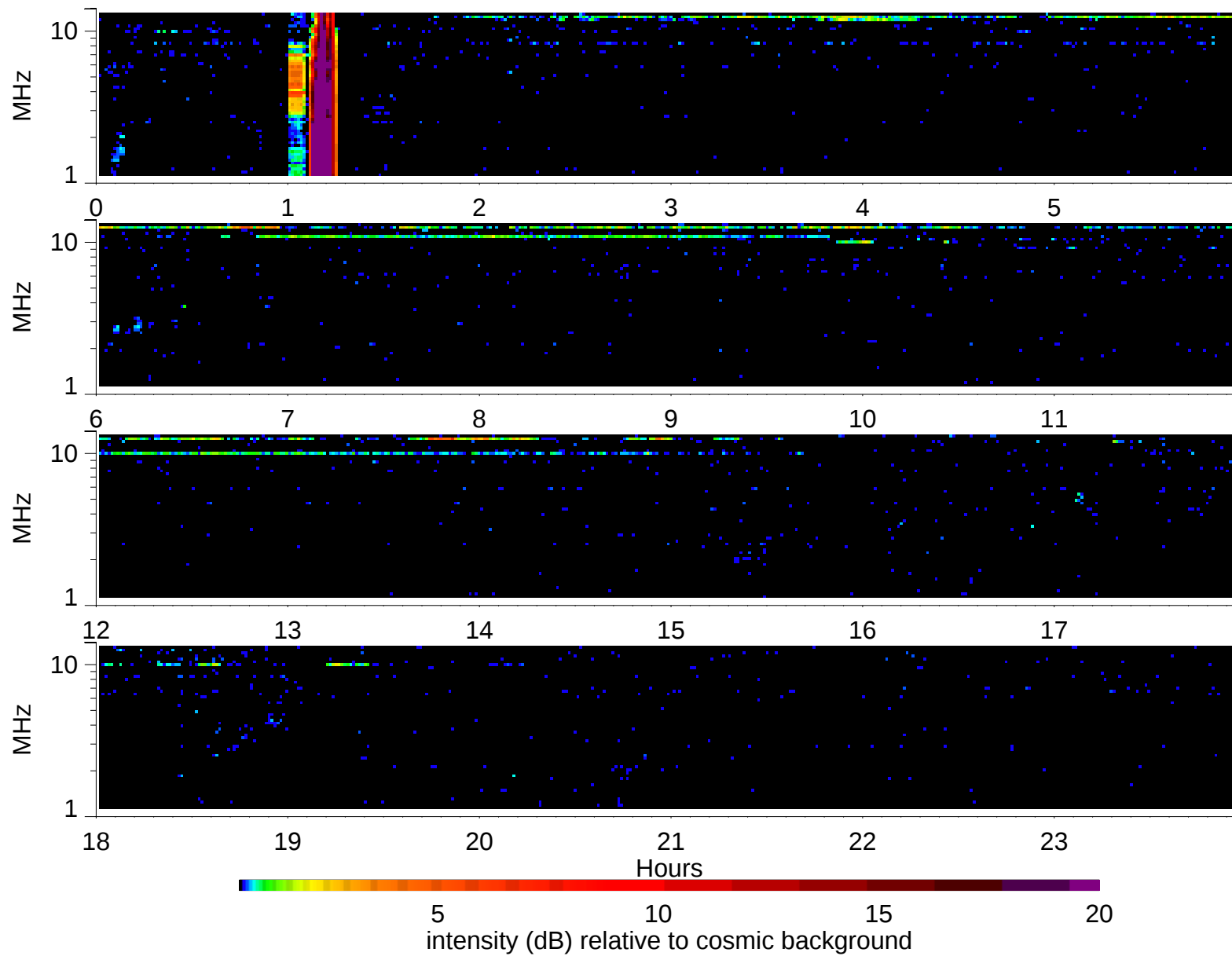
Wind Waves RAD2 receiver: 1997/2/13
