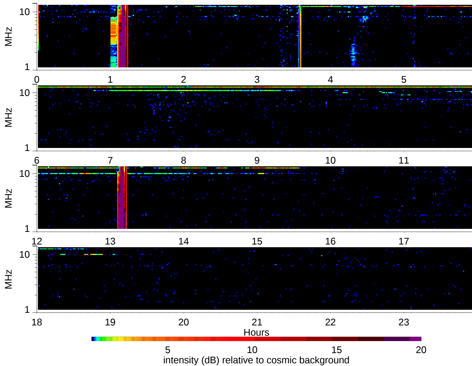
Wind Waves RAD2 receiver: 1997/2/15
