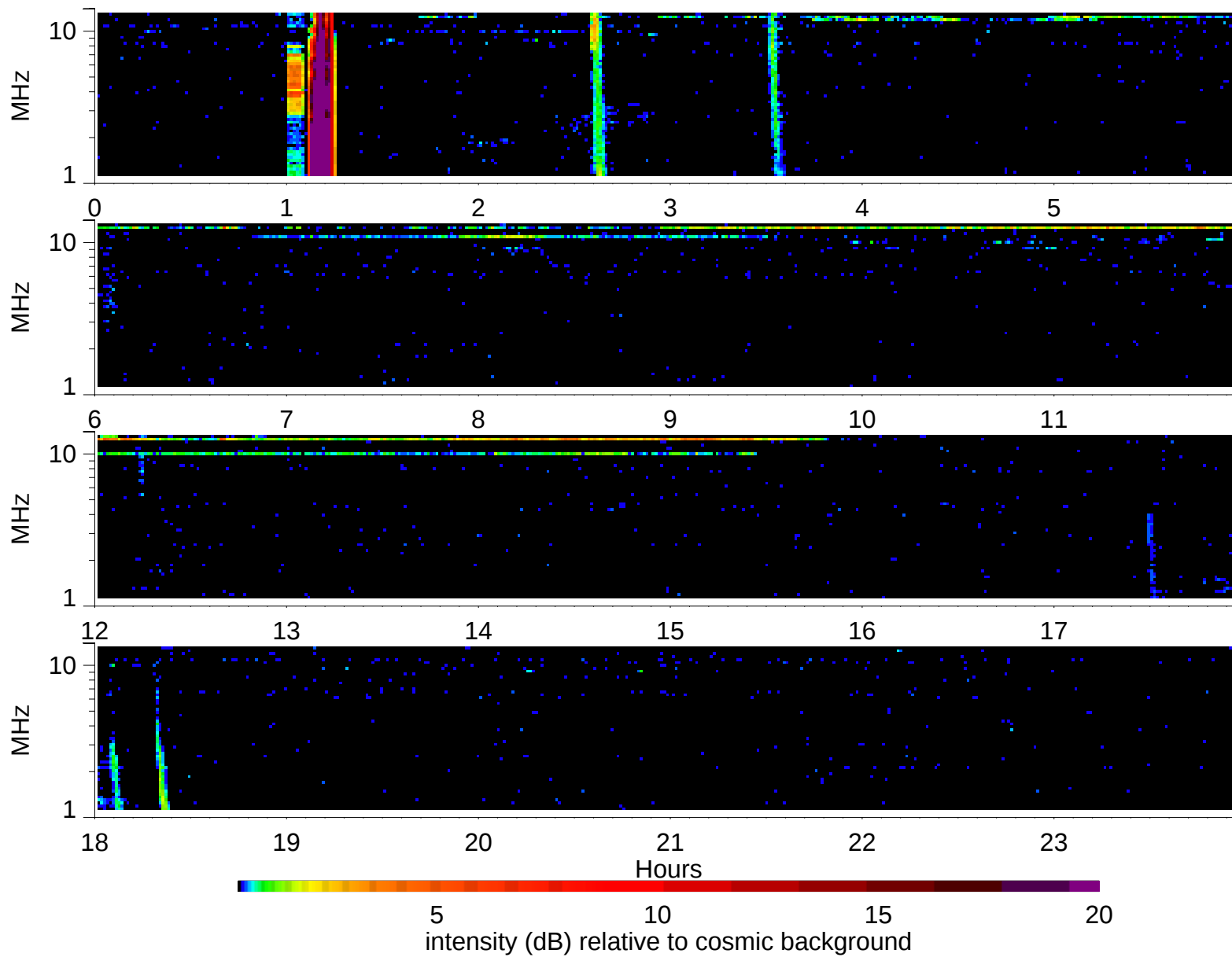
Wind Waves RAD2 receiver: 1997/2/21
