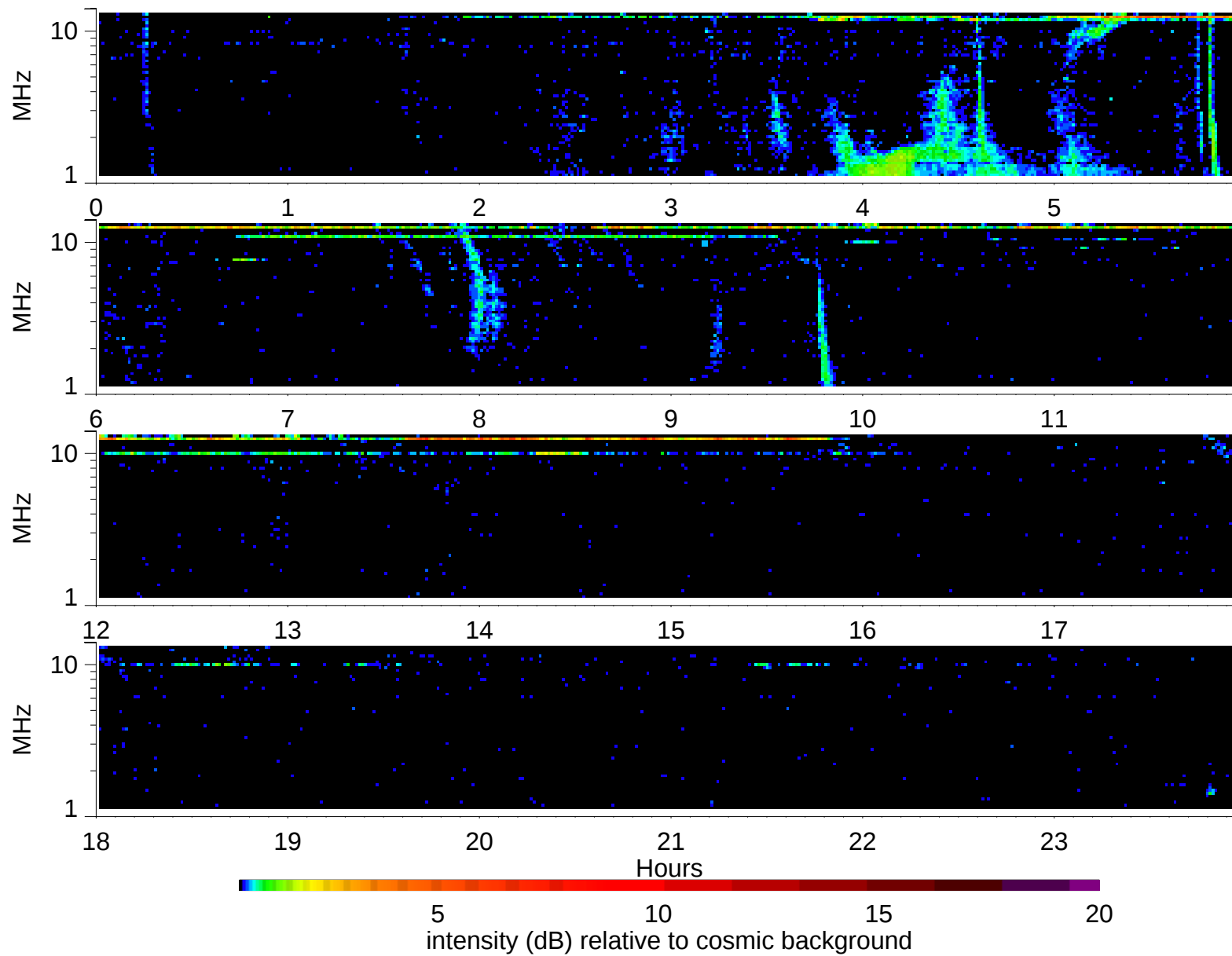
Wind Waves RAD2 receiver: 1997/2/22
