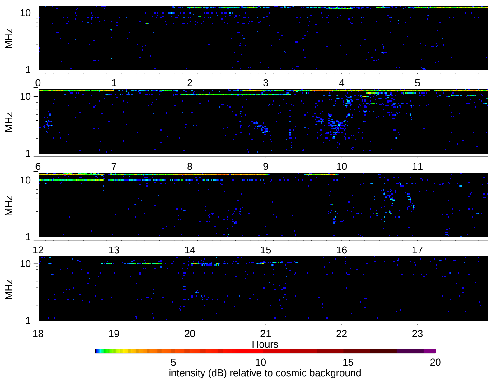
Wind Waves RAD2 receiver: 1997/2/24
