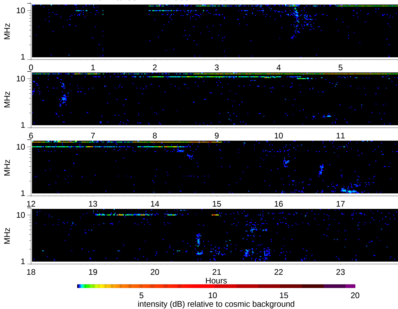
Wind Waves RAD2 receiver: 1997/2/26
