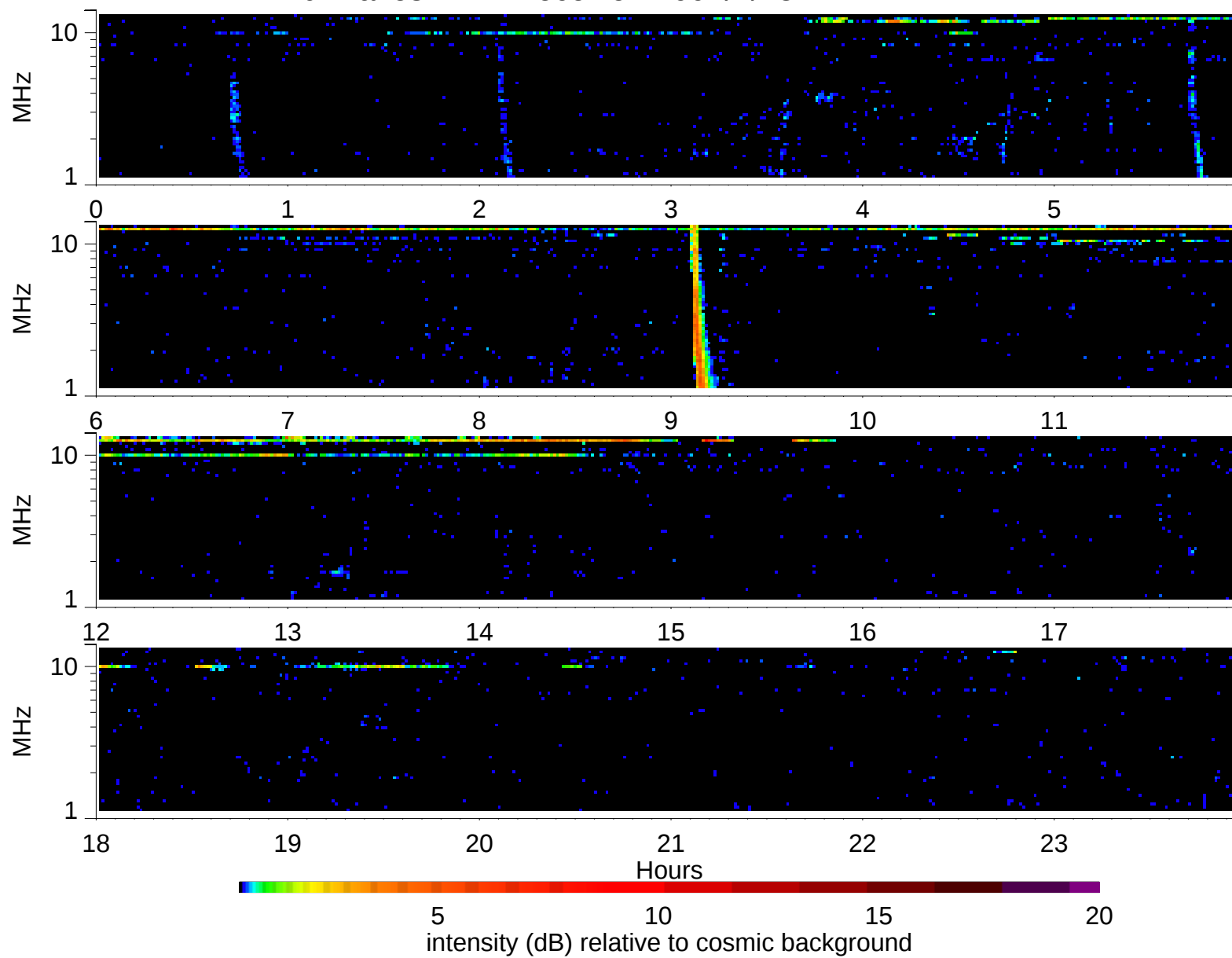
Wind Waves RAD2 receiver: 1997/2/28
