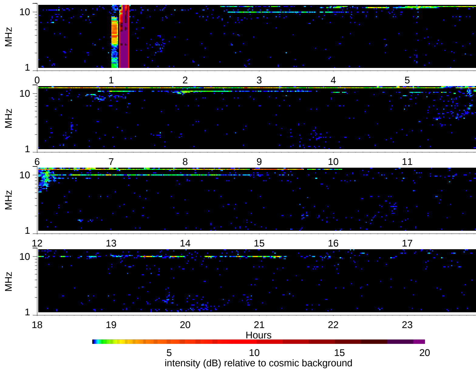
Wind Waves RAD2 receiver: 1997/3/3
