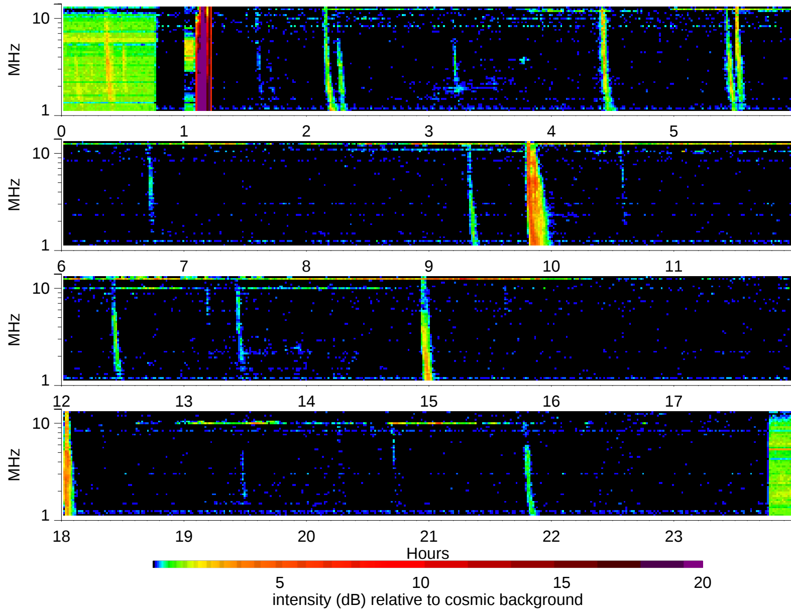
Wind Waves RAD2 receiver: 1997/3/7
