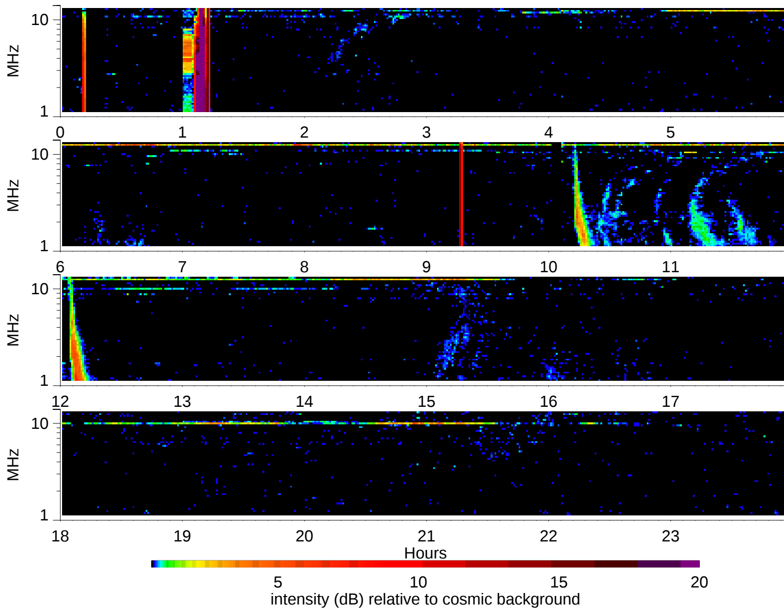
Wind Waves RAD2 receiver: 1997/3/15
