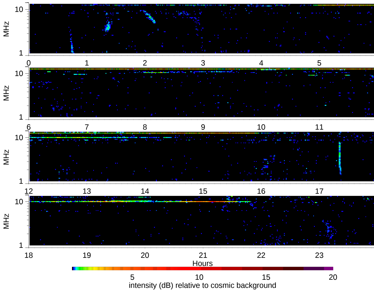
Wind Waves RAD2 receiver: 1997/3/16
