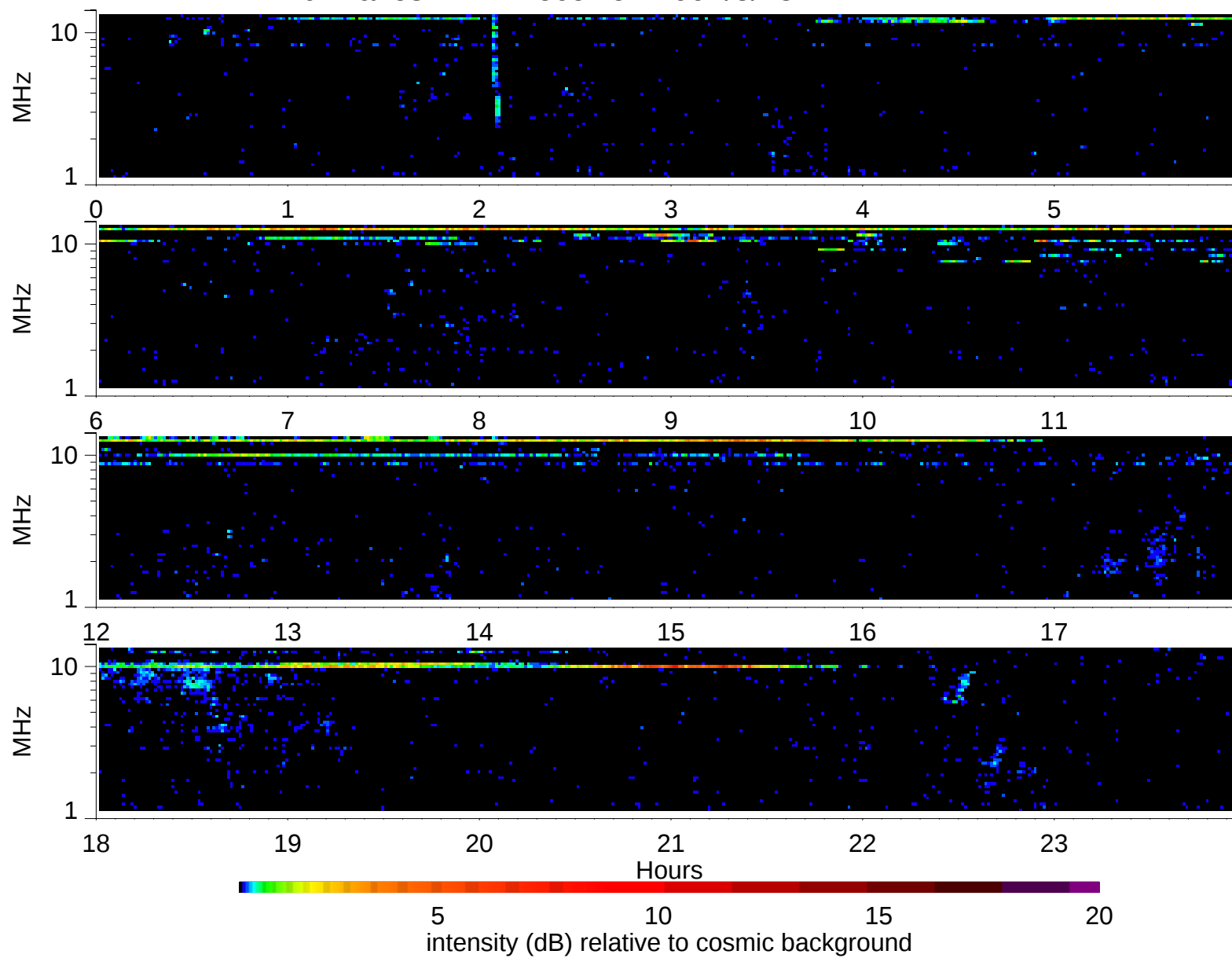
Wind Waves RAD2 receiver: 1997/3/18
