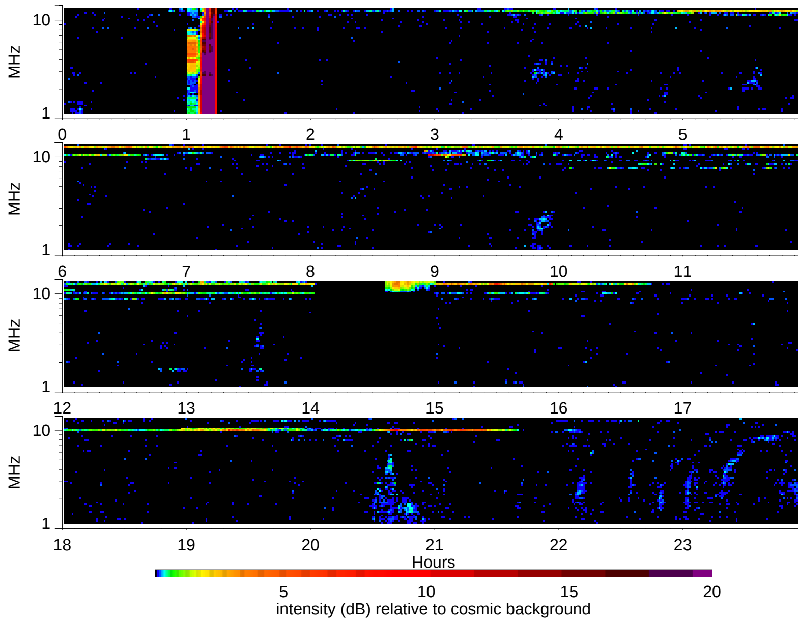
Wind Waves RAD2 receiver: 1997/3/19
