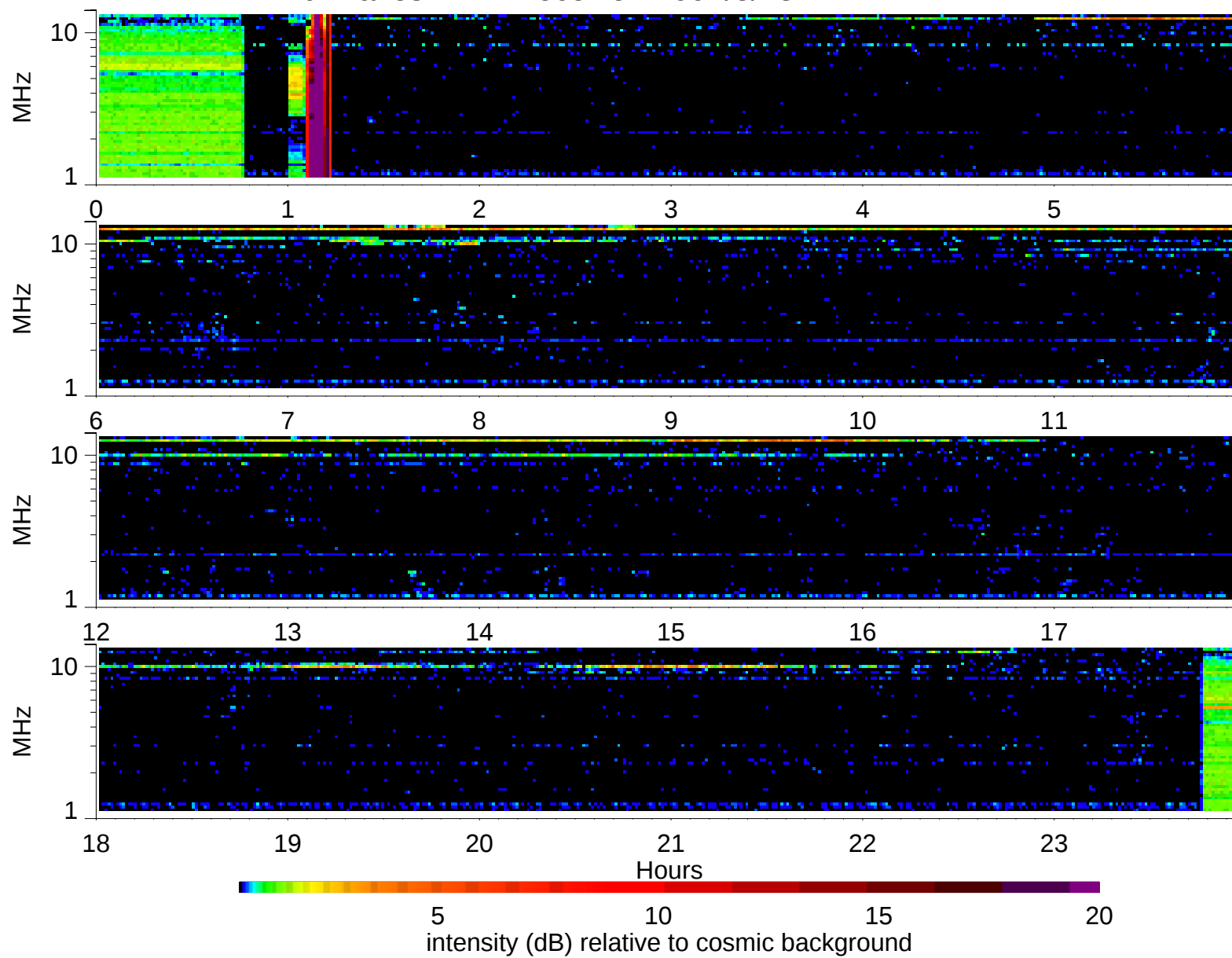
Wind Waves RAD2 receiver: 1997/3/23
