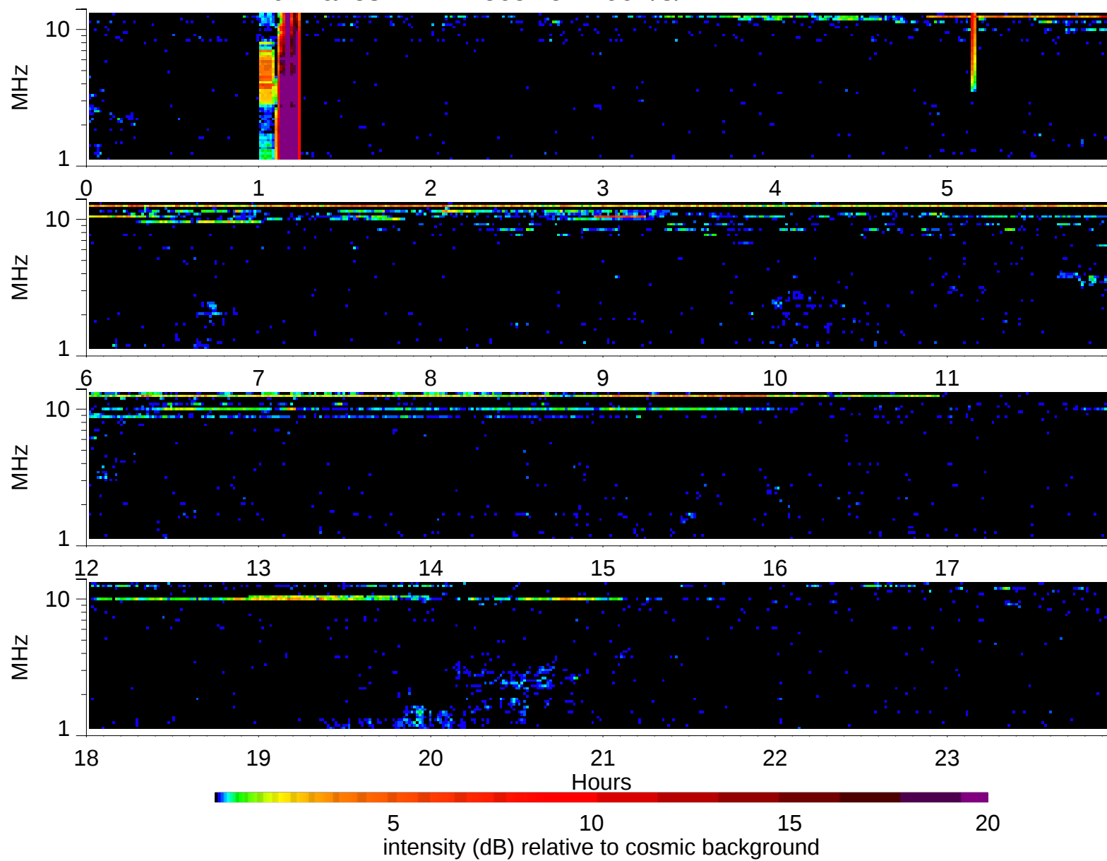
Wind Waves RAD2 receiver: 1997/3/27
