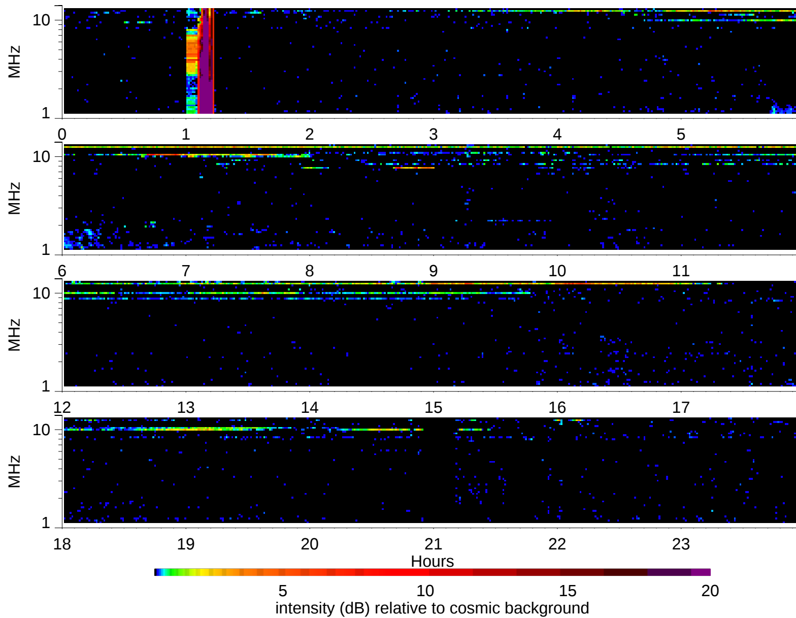
Wind Waves RAD2 receiver: 1997/4/6
