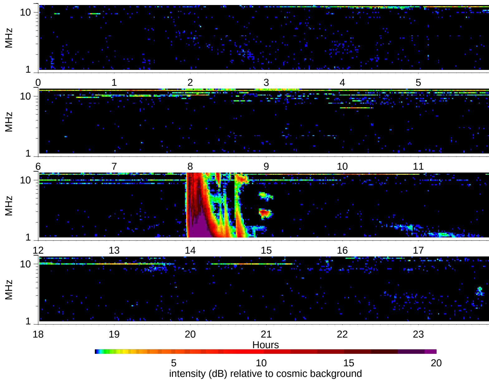
Wind Waves RAD2 receiver: 1997/4/7
