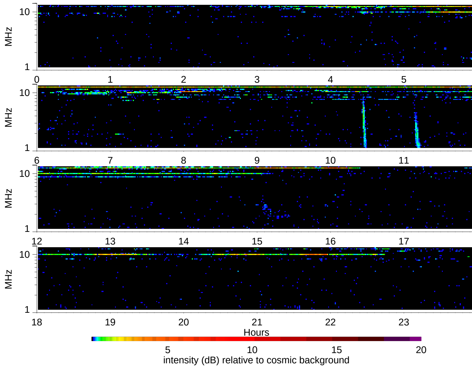
Wind Waves RAD2 receiver: 1997/4/9
