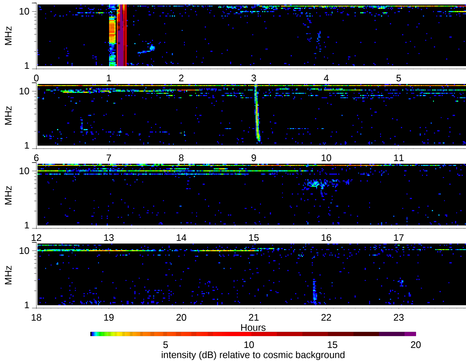
Wind Waves RAD2 receiver: 1997/4/10
