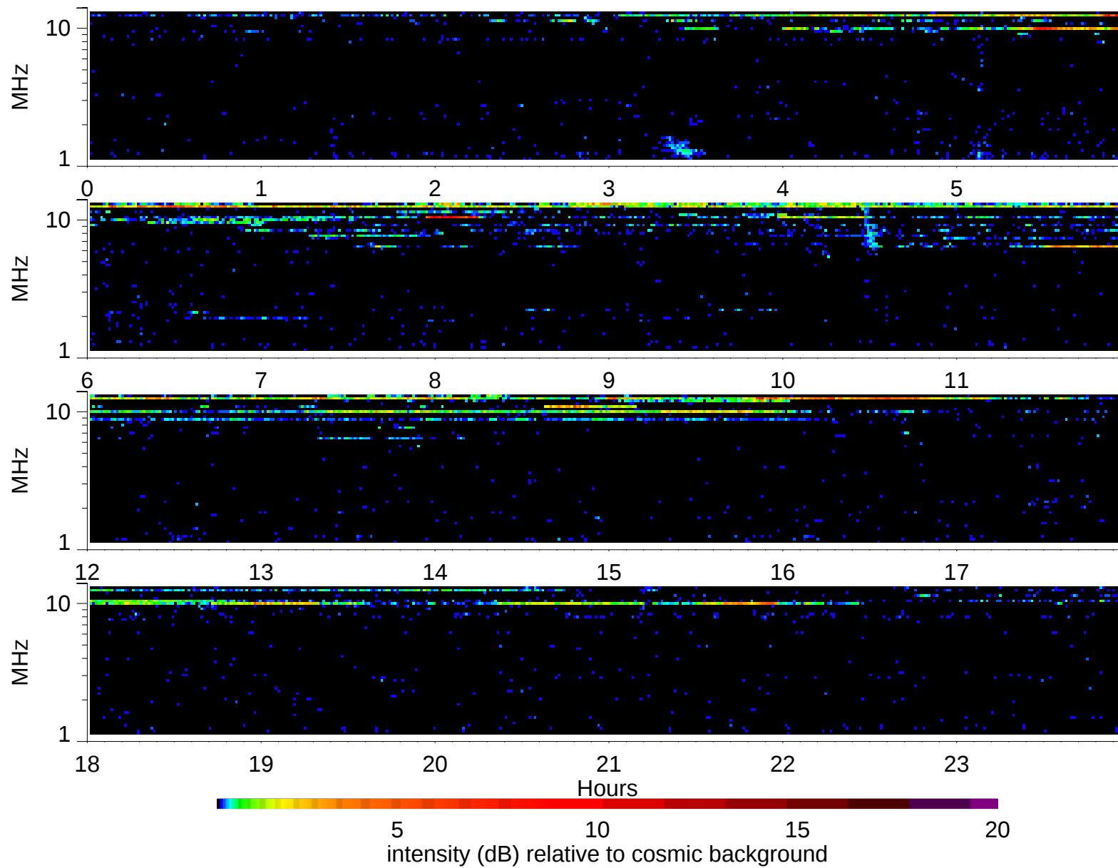
Wind Waves RAD2 receiver: 1997/4/11
