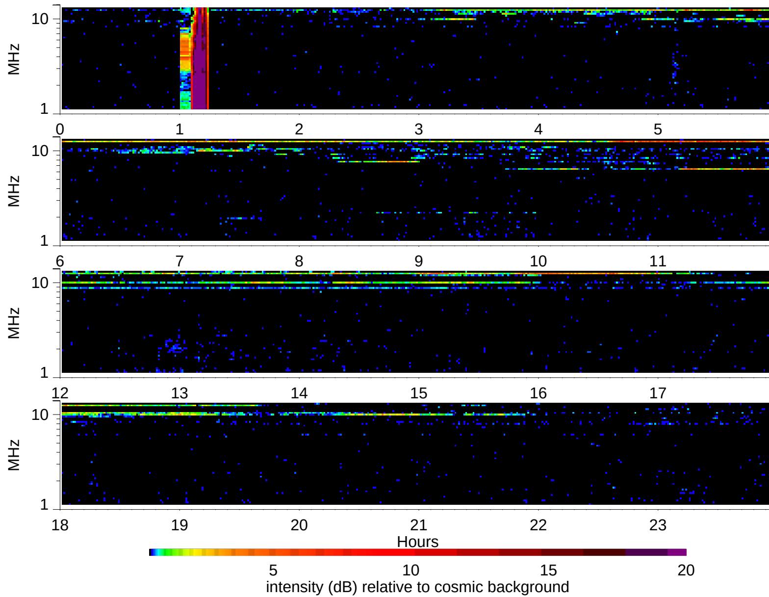
Wind Waves RAD2 receiver: 1997/4/12
