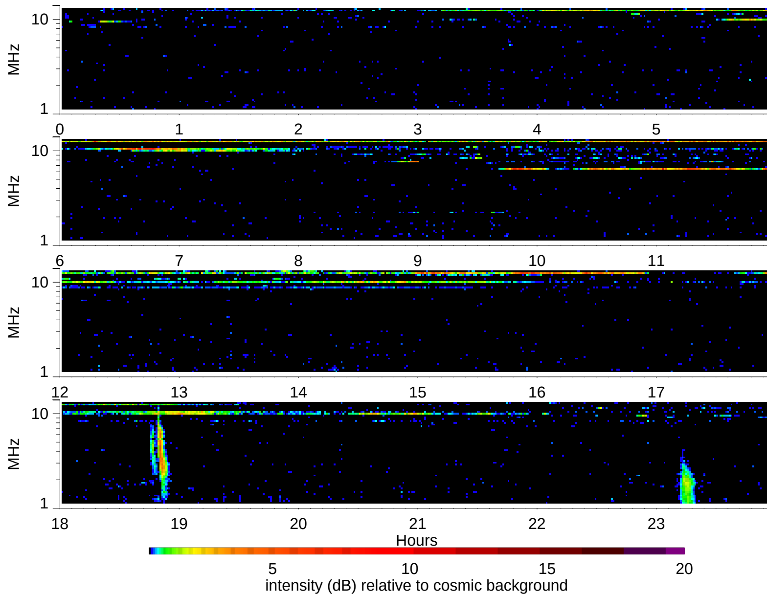
Wind Waves RAD2 receiver: 1997/4/13
