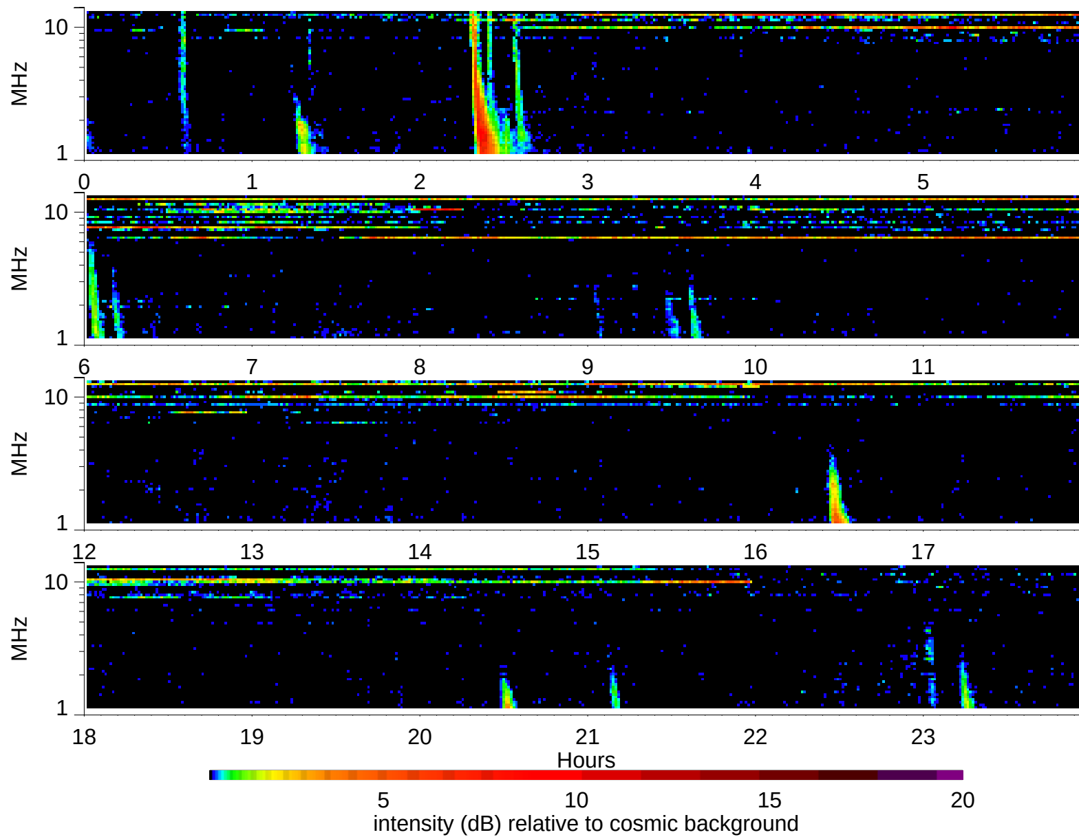
Wind Waves RAD2 receiver: 1997/4/17
