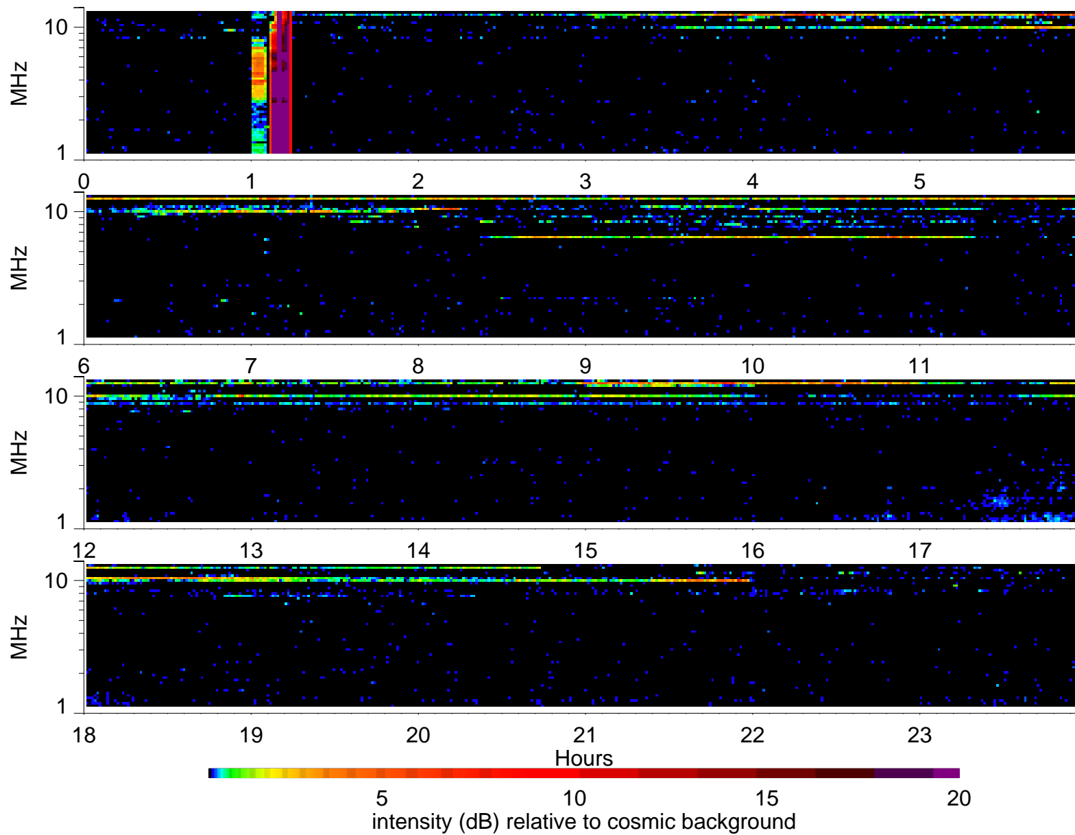
Wind Waves RAD2 receiver: 1997/4/18
