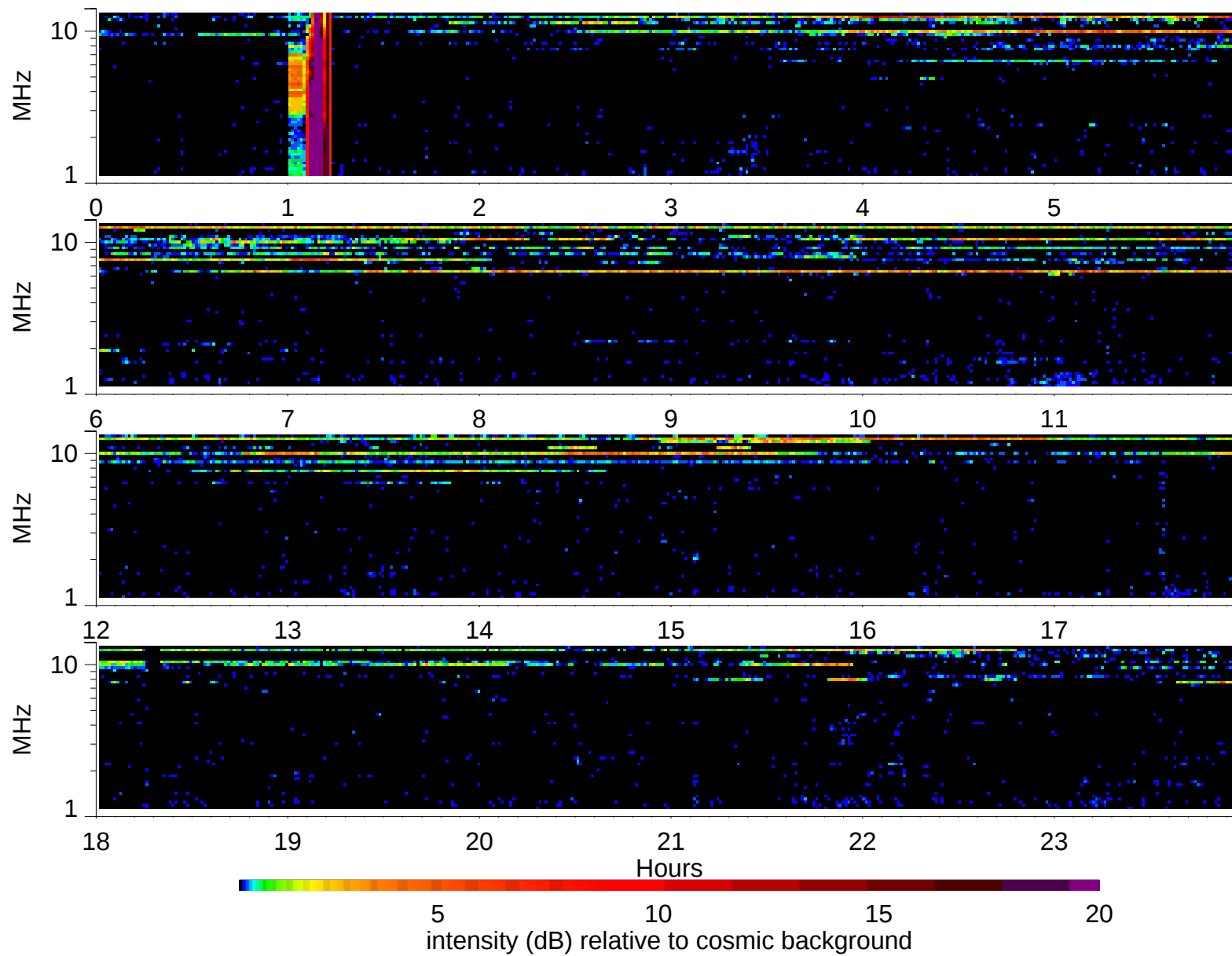
Wind Waves RAD2 receiver: 1997/4/22
