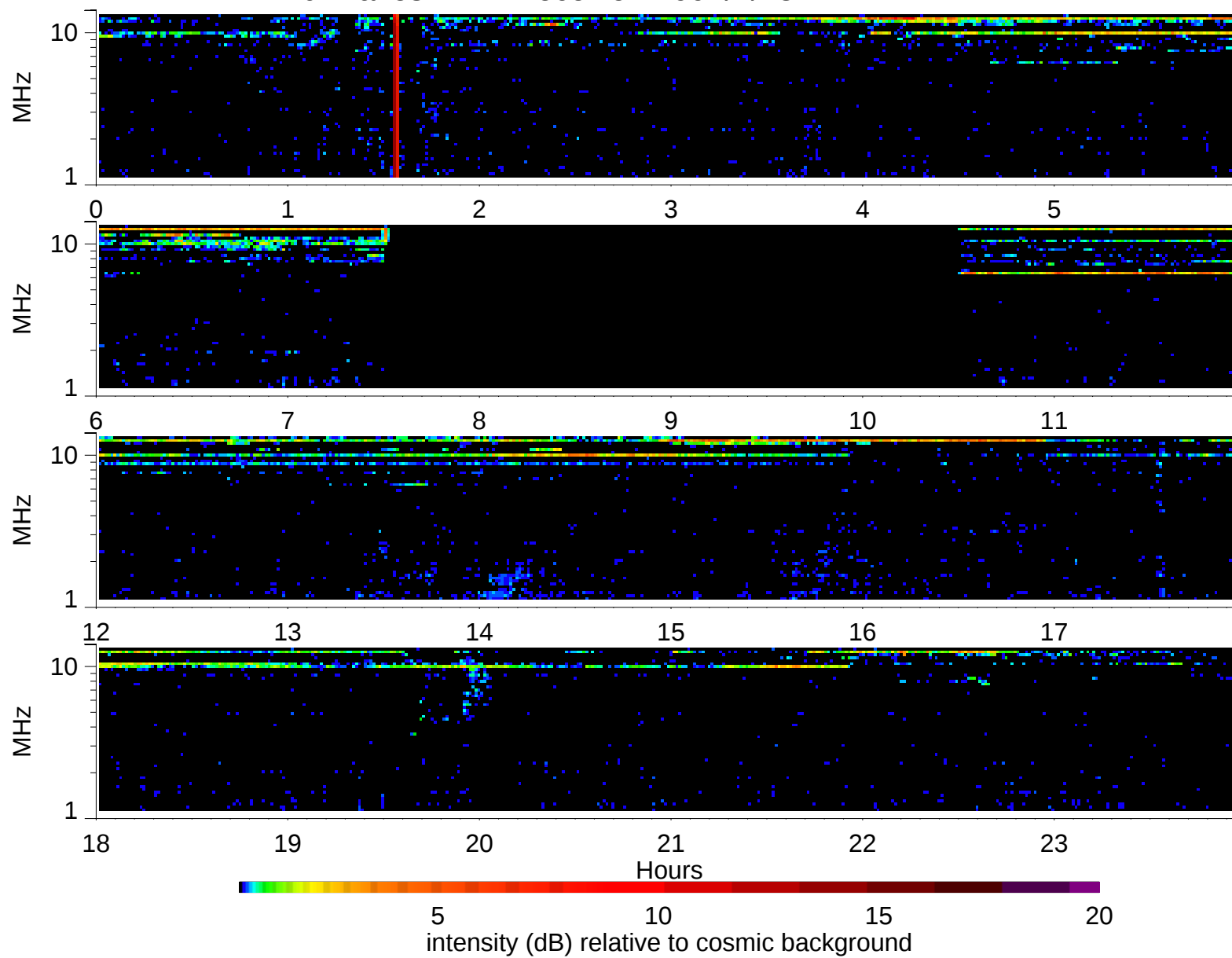
Wind Waves RAD2 receiver: 1997/4/23
