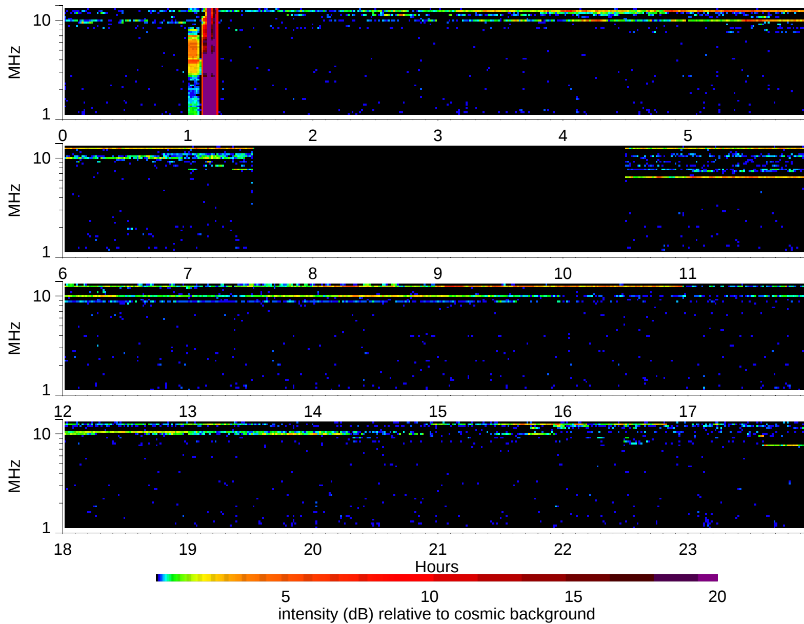
Wind Waves RAD2 receiver: 1997/4/26
