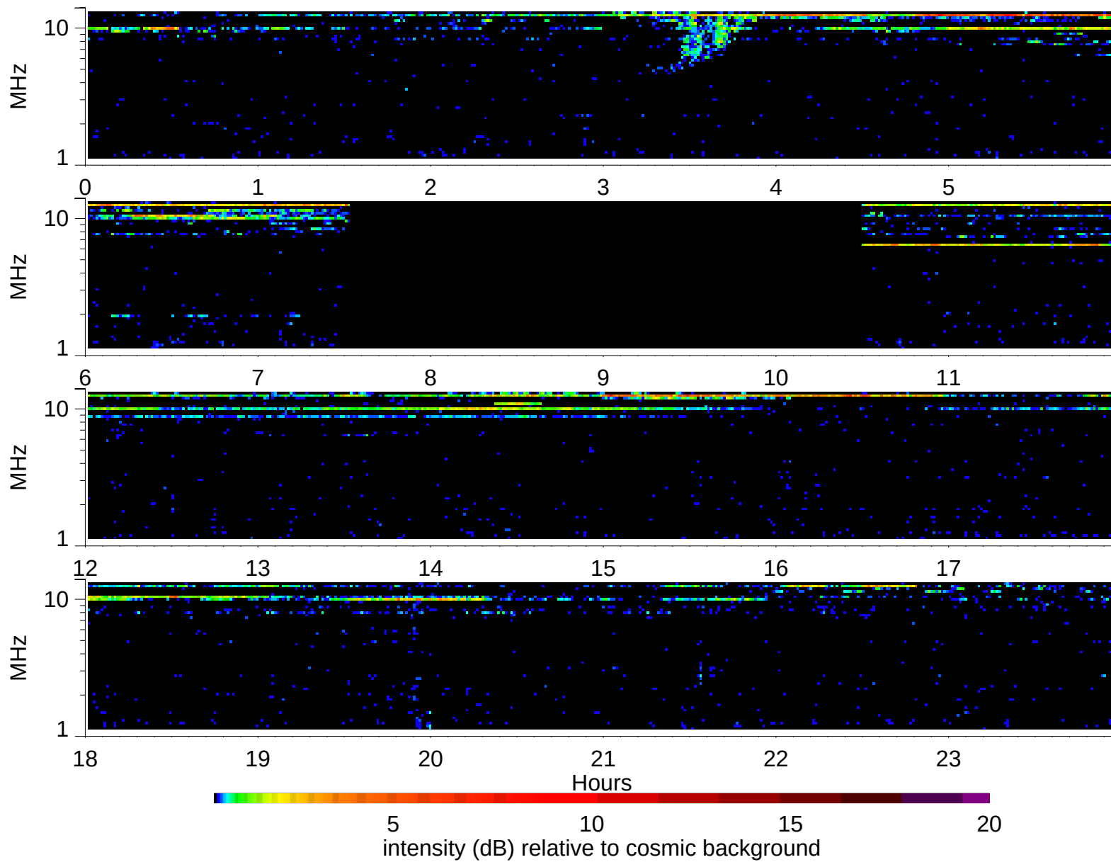
Wind Waves RAD2 receiver: 1997/4/29
