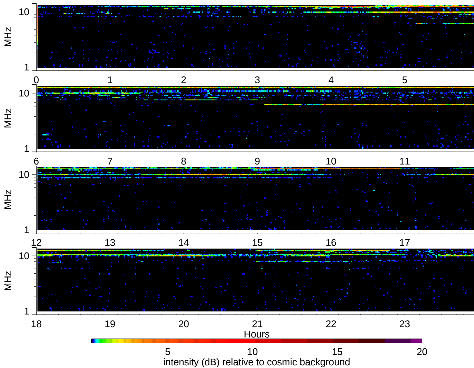
Wind Waves RAD2 receiver: 1997/5/3
