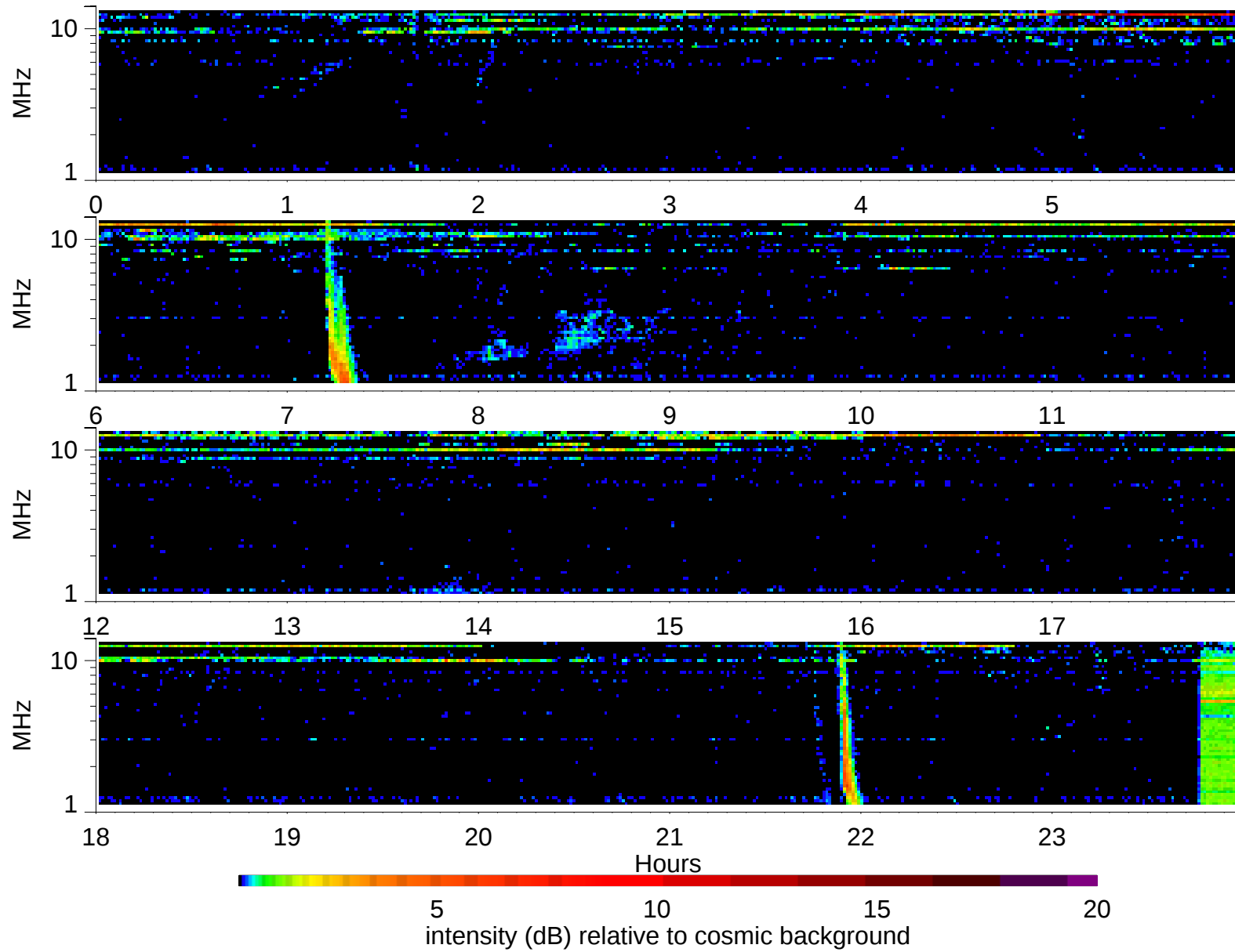
Wind Waves RAD2 receiver: 1997/5/7
