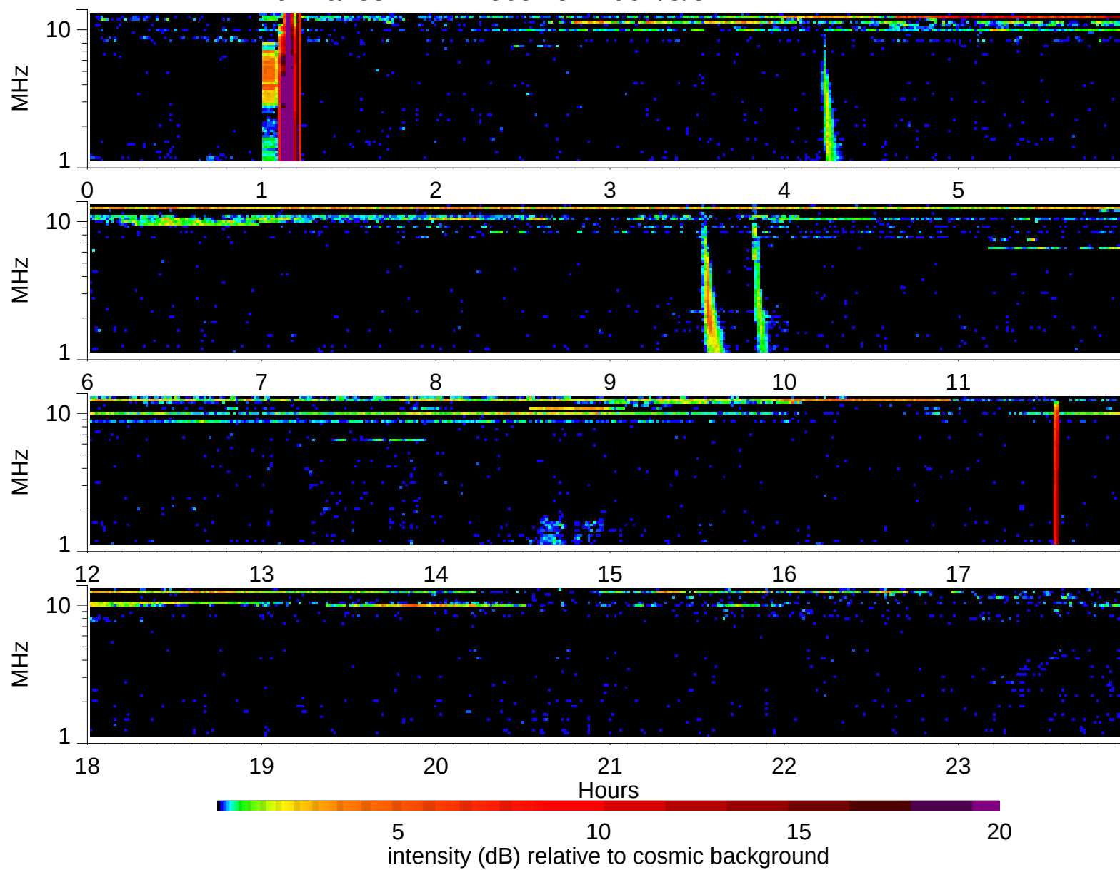
Wind Waves RAD2 receiver: 1997/5/8
