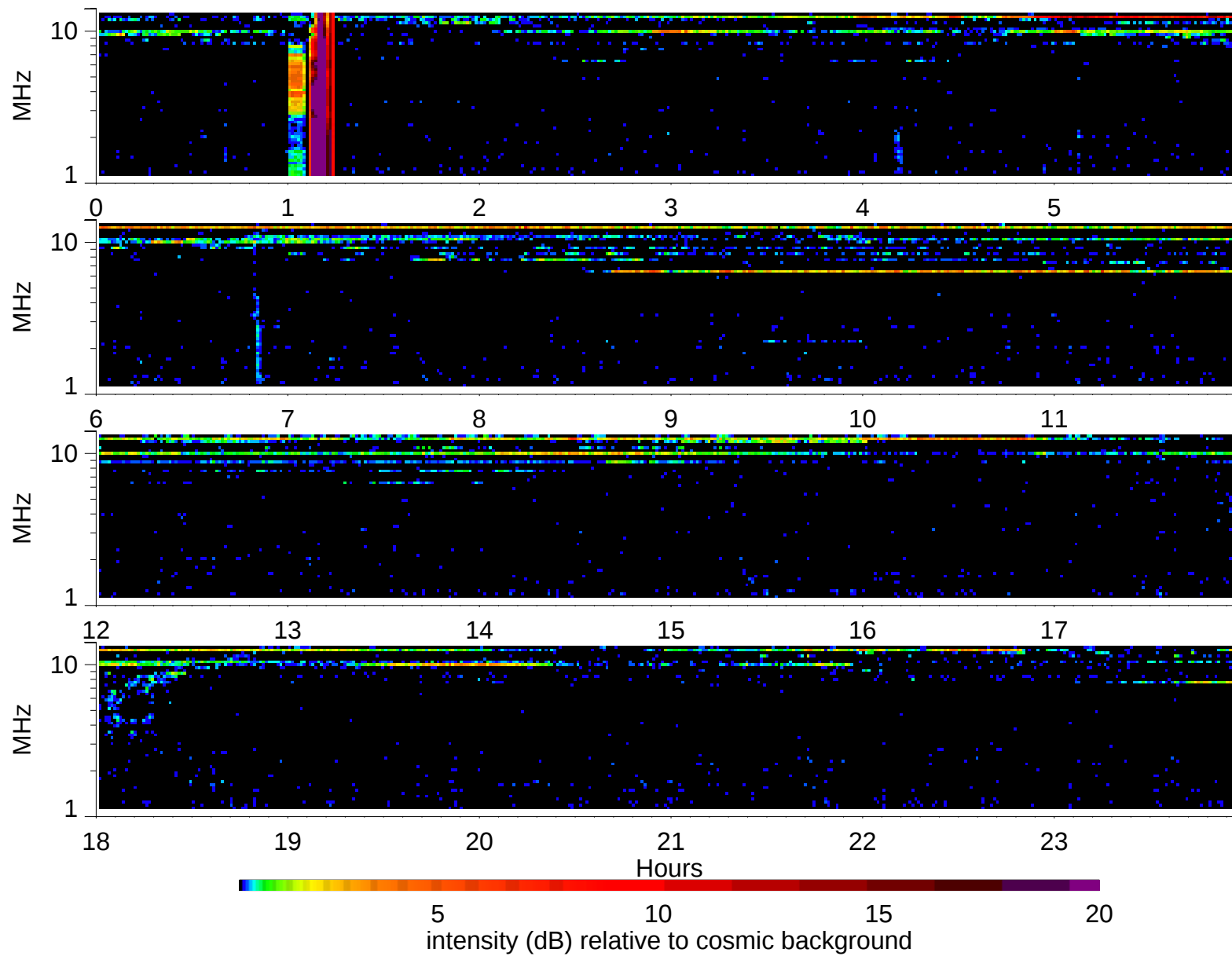
Wind Waves RAD2 receiver: 1997/5/10
