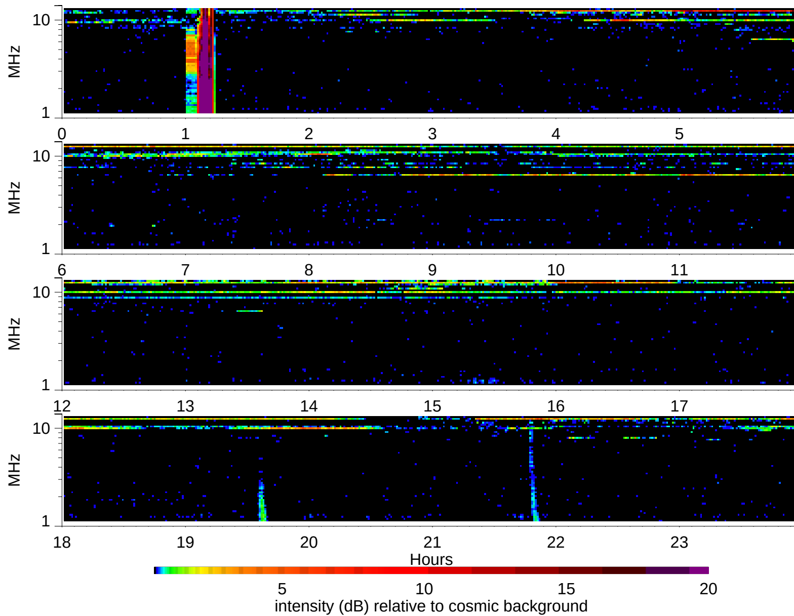
Wind Waves RAD2 receiver: 1997/5/14
